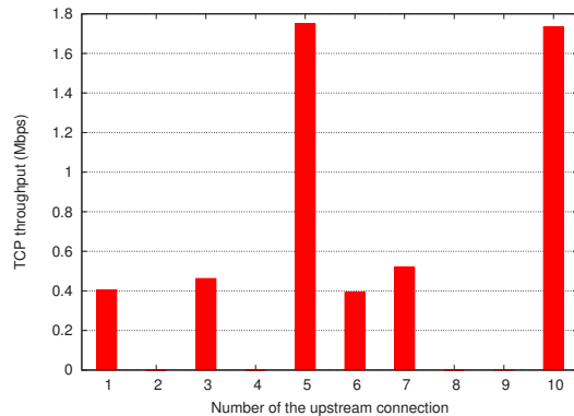
Fig. 1. Competing TCP uploads, 10 stations (NS2 simulation, 802.11 MAC, 300s duration, parameters as in Table I).
