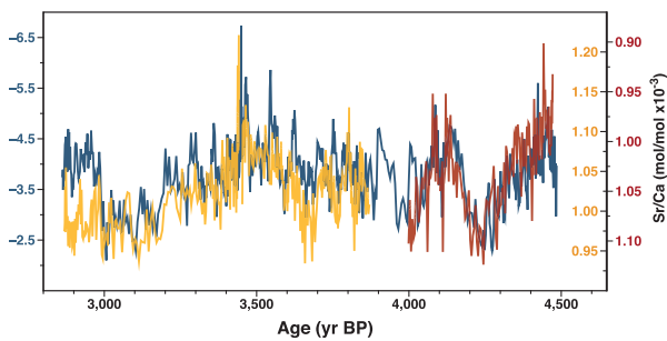
Figure 4. Comparison of AB13 \delta^{18}\text{O} and Sr/Ca time series. Note that the scale for the Sr/Ca data reverses from increasing downwards for the older portion of the record (4.6 ky BP to 4.0 kyBP), red in color, to increasing upwards for the remainder of the record, orange/yellow in color.
