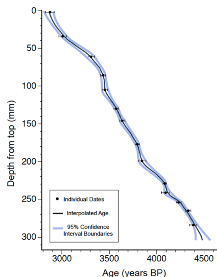
Figure 2. Age model for stalagmite AB13. Black line represents interpolated median ages between individually dated subsamples, black dots indicate individual dates, and blue highlight indicates 95% CI low and high boundaries. (COPRA source code available at https://tocsy.pik-potsdam.de/copra.php ).
