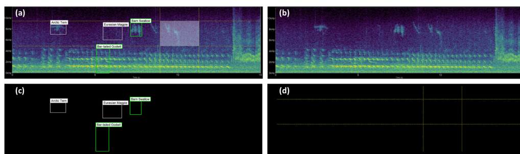
Figure 3 Spectrogram plot. The full spectrogram plot (A) is a combination of overlapping panels. From back to front: (B) highlights the main spectrogram, which is the slowest to render; (C) shows the labels panel displaying bounding box annotations; and (D) emphasizes the time/frequency guides which gauge the time and frequency ranges the sound clip occupies, as well as tracing the shape of the bounding box should a label be saved.
