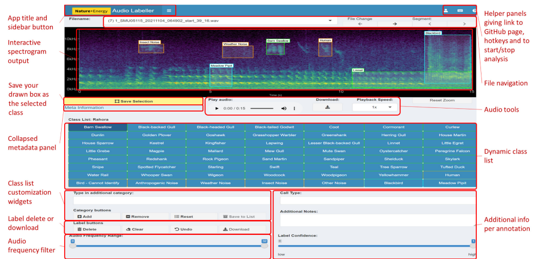
Figure 1 Main components of the App User Interface. The main interactive element of the app is the spectrogram, providing a visual representation of the sound. This plot can be drawn on with boxes to filter audio or make annotations. The button on the left underneath the spectrogram is for saving the current selection on the plot, which will be labelled with the class from the grid of categories below. Various audio playback widgets are grouped together to the right of the save button. File navigation allows the user to proceed to the next file in the workflow folder, or select from a drop-down menu of available files, the second of which displays the number of annotations present in each file. The collapsed side panel on the left hand side has extra configuration settings expected to be changed at most once or twice per session. The class list is dynamic: the core (green) categories are selected from a drop-down list in the Configuration tab, while the miscellaneous (orange) categories are static in the current implementation. Custom categories can be added or removed using the category widgets below. Users can provide more information than just the primary category (e.g., bird species) of sound identified; these can include call type, free text additional notes and label confidence.
