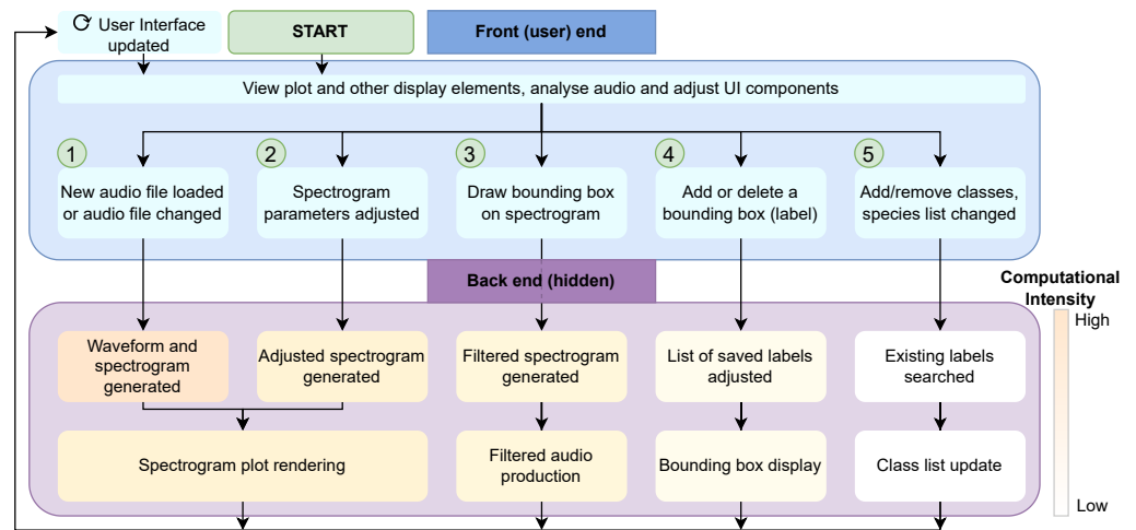
Figure 2 Workflow diagram. Demonstration of the front and back-end workflow of the NEAL app. Any analyses or adjustments carried out by the user in the user interface affect the relevant processes in the back end. This keeps the user focused only on the elements being updated while reducing downtime compared to the event that the entire page is refreshed every time. Each of the steps ① to ⑤ in the front end—the actions and changes performed by the user via the UI—have corresponding processes in the back-ground which are in decreasing order of computational demand. The advantage is that these back-end processes have little to no overlap, meaning they can be run separately when the front-end changes are unrelated. If the change is minor (far right, in white) we do not want this to result in an avoidable refresh involving large computations (shown to the left of the figure in orange).
