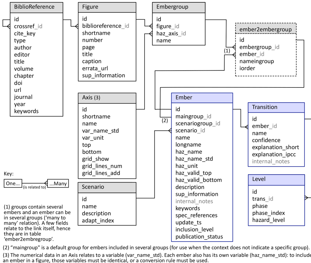
Figure 2. Database tables, fields, and relationships, focusing on the main content (excluding user accounts providing editing access rights and other technical details). Tables with a blue frame store the assessment of risk changes shown in embers diagrams, and the other tables provide additional information on how this content should be illustrated and where it appears in IPCC reports. The names prefixed by haz_ relate to “hazard”, that is, the variable used as the climate change metric ( y axis of the embers). Greyed-out fields are editors only (see Sect. 2.5). All variables are described in Sect. S1.1 in the Supplement.
