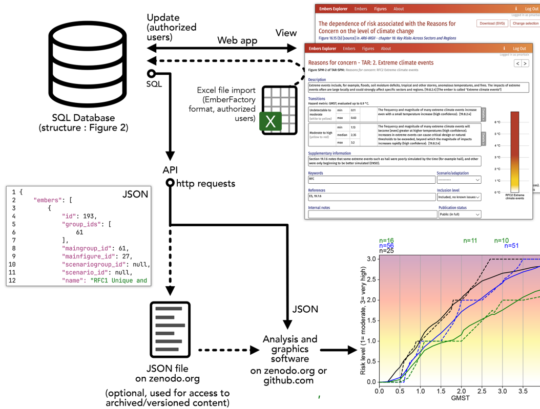
Figure 3. Schematic view of data access options. Each field in the database and JSON files is described in Sect. S1.
