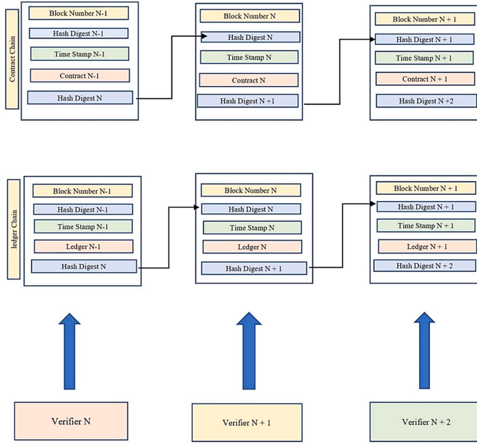
Fig. 4. Blockchain-based transaction settlement.
