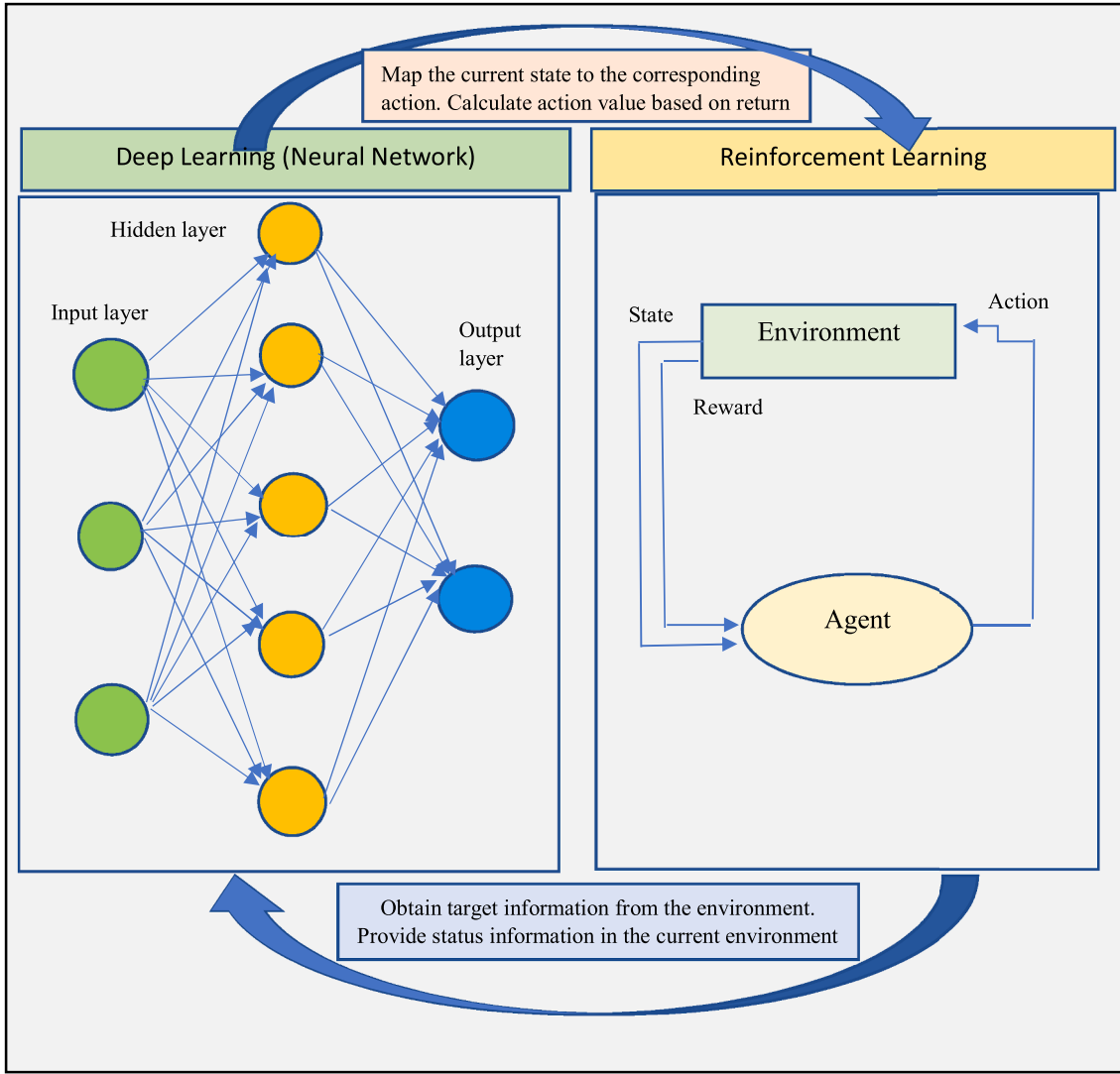
Fig. 5. Feedforward neural network with reinforcement learning.
