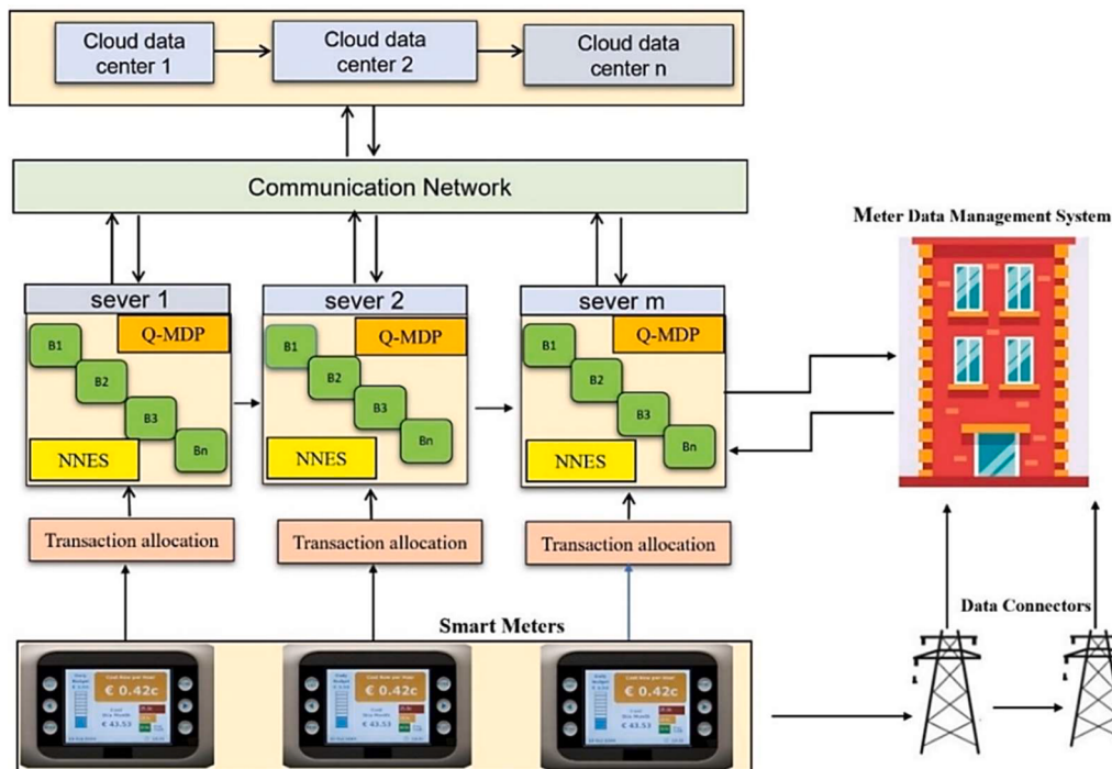
Fig. 2. Three-Tier Architecture.
