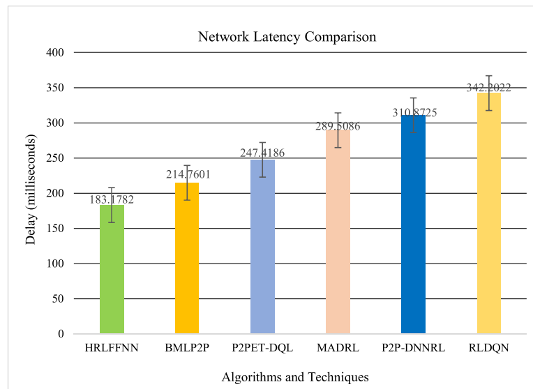
Fig. 15. State-of-the-art techniques comparison for network latency.
