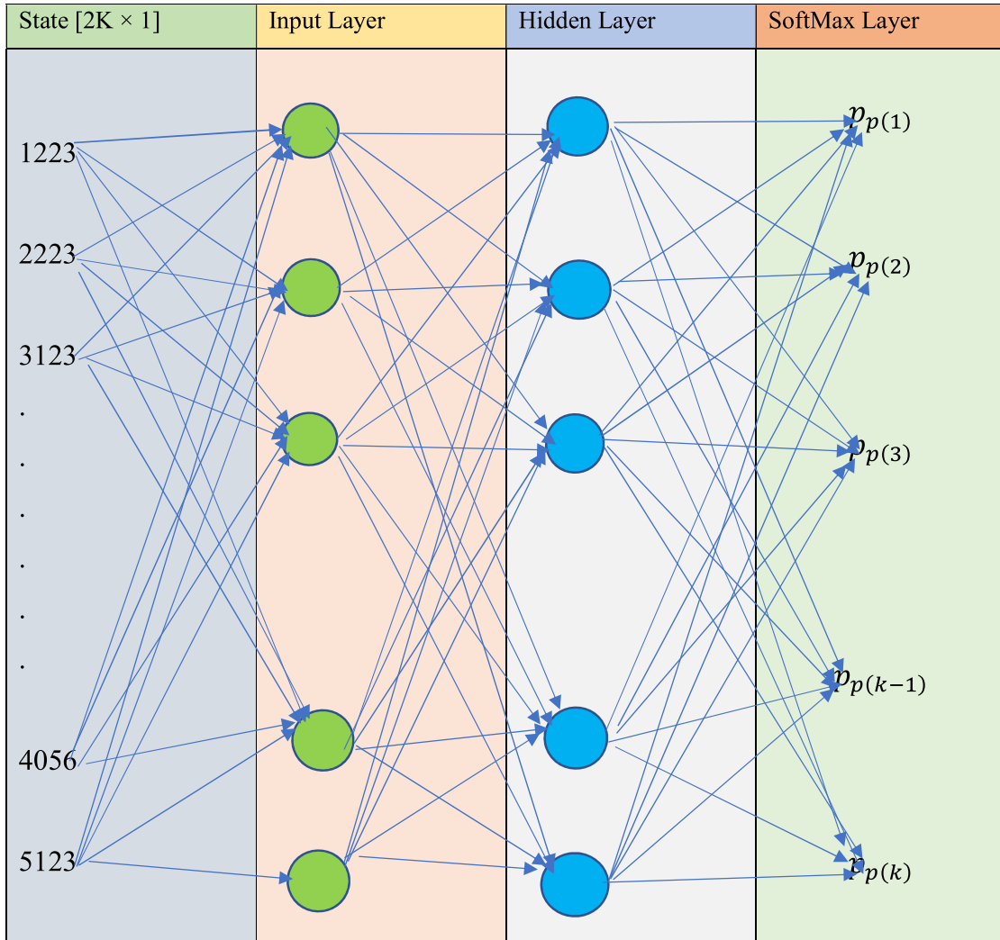
Fig. 6. The FFNN states and layers.
