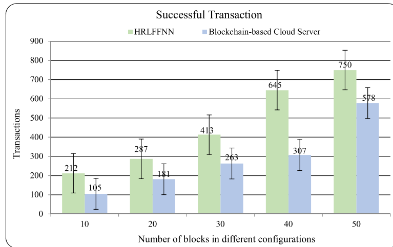
Fig. 12. PoW for successful transaction in the proposed algorithm and blockchain-based cloud.
