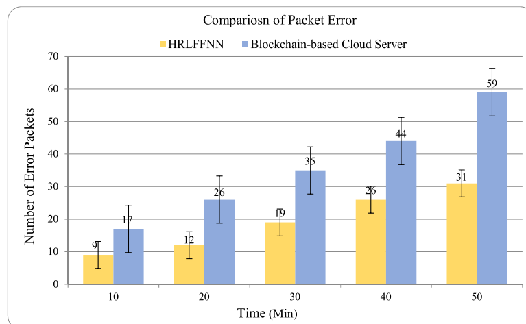
Fig. 14. Packet error comparison in the proposed algorithm and blockchain-based cloud.
