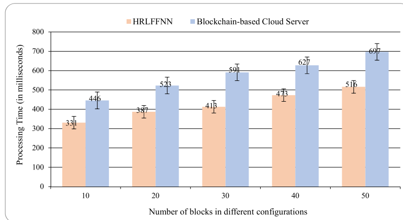
Fig. 13. Processing time comparison for the proposed algorithm and blockchain-based cloud.
