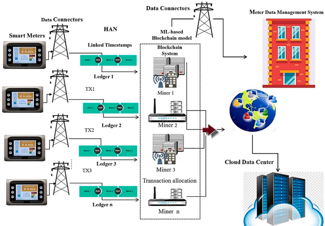
Fig. 3. Advanced machine learning-based blockchain model.
