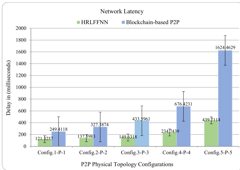
Fig. 11. Network latency comparison for the proposed algorithm and the blockchain-based cloud.
