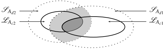
Fig. 2. Two Padé approximations.
