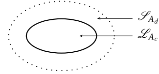
Fig. 1. Illustration of Theorem 1.
