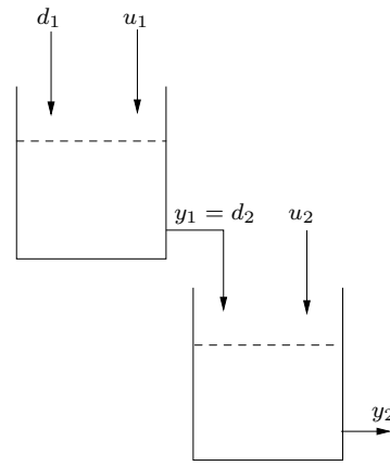
Fig. 3. Schematic diagram of a two-stage pH-neutralization process.
