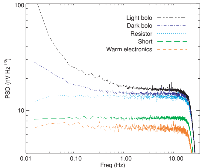
Figure 34. PSD of the noise from various sources. “Warm electronics” accounts for both the readout and the bias generator and was made by connecting a warm 1 k \Omega resistor in place of the cold bolometers and amplifiers. “Short” is a measurement of the noise across a short located on the focal plane and includes contributions from the cold JFETS and the warm amplifiers (but not the bias generator). “Resistor” is a properly biased 10 M \Omega resistor on the focal plane. “Dark bolo” is the readout from a dark bolometer. “Light bolo” is the readout from a 150 GHz bolometer made during normal operation and includes contributions from atmospheric 1/f .
