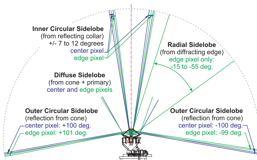
Figure 27. Schematic showing the location and origin of the telescope sidelobes. (A color version of this figure is available in the online journal.)
