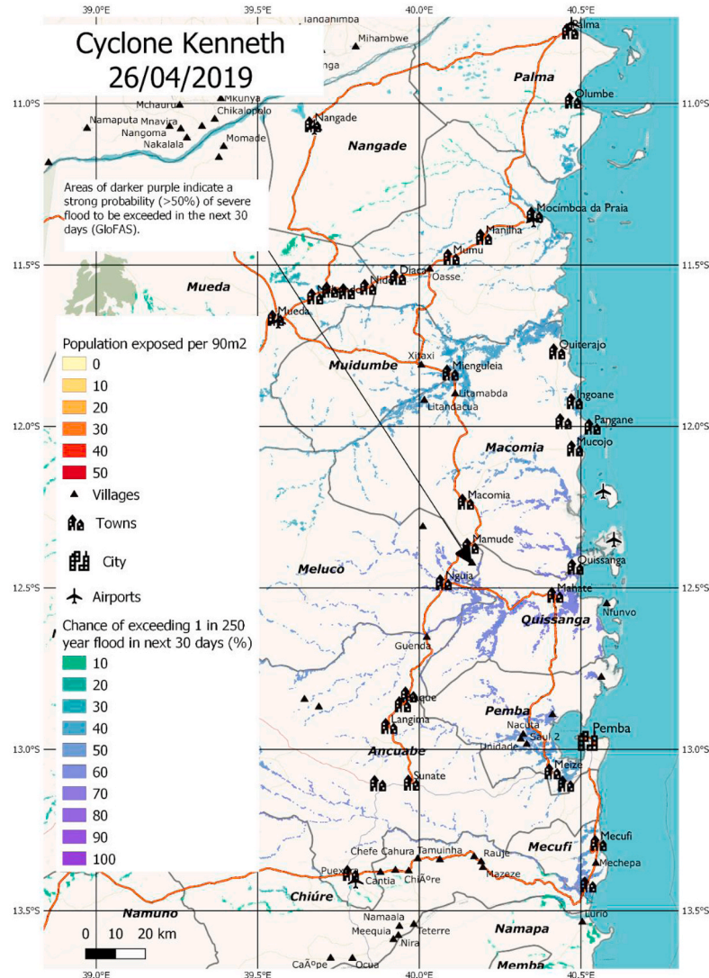
Figure 7: Flood hazard map of Mozambique (mostly Cabo Delgado Province). The probability of flooding exceeding the severe flood level (250-year return period) over the next 30 days is shown in purple. Potentially exposed population is shown in red by district.
