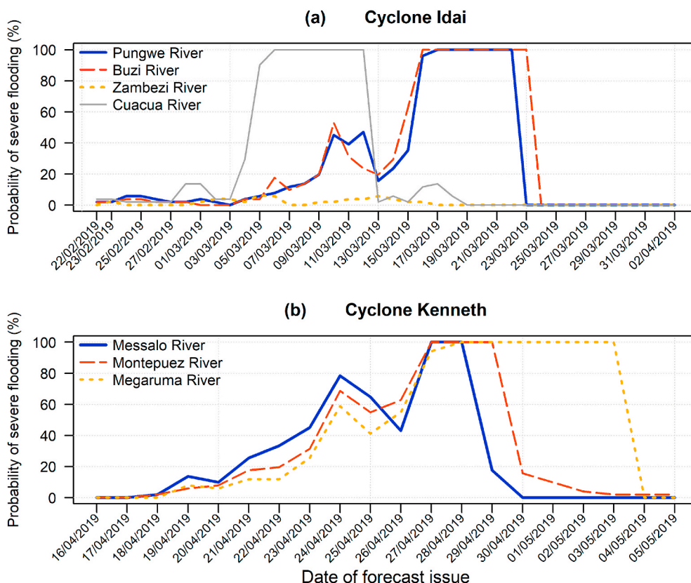
Fig. 6. GloFAS maximum probability of exceeding the severe flood alert threshold (20-year return period/5% AEP) during the 30-day forecast horizon, for major rivers affected by (a) Cyclone Idai and (b) Cyclone Kenneth, for forecasts issued daily ahead of and during each cyclone. The rivers and locations (see Fig. 3) shown are (a) Pungwe at Mafambisse (15 km northwest of Dondo), Buzi at Buzi, Zambezi at Tete, Cuacua at Campo (Mopeia district, 50 km west of Quelimane), and (b) Messalo at Narere (60 km north of Macomia), Montepuez at Quis-sanga district (45 km southeast of Macomia) and Megaruma at Chiúre district (12 km south of Mecúfi).
