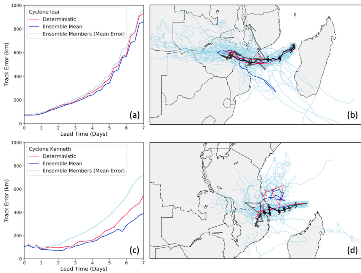
Fig. 7. Track location errors with lead time for ECMWF forecasts of Cyclones (a) Idai and (c) Kenneth. Errors are the mean error across all forecasts (produced twice daily at 00 and 12 UTC) for the tropical cyclone stages of each storm, for the high-resolution deterministic (red) and ensemble mean (dark blue) forecasts, and the mean error across all 50 individual ensemble members (light blue). Forecast tracks are verified against the IBTrACS observed best tracks. An example forecast for Cyclone Idai is shown in (b), issued on 10th March 2019 at 00 UTC, and for Cyclone Kenneth in (d), issued on 23rd April at 12UTC. These maps indicate the forecast track for the deterministic (red) and all 50 individual ensemble members (light blue), alongside the track of the ensemble mean (dark blue). The observed tracks of Cyclones Idai and Kenneth are shown in black, where tropical cyclones symbols denote the cyclone-strength stages of the storm, followed by a grey solid line representing the post-cyclone stages. (For interpretation of the references to colour in this figure legend, the reader is referred to the Web version of this article.)
