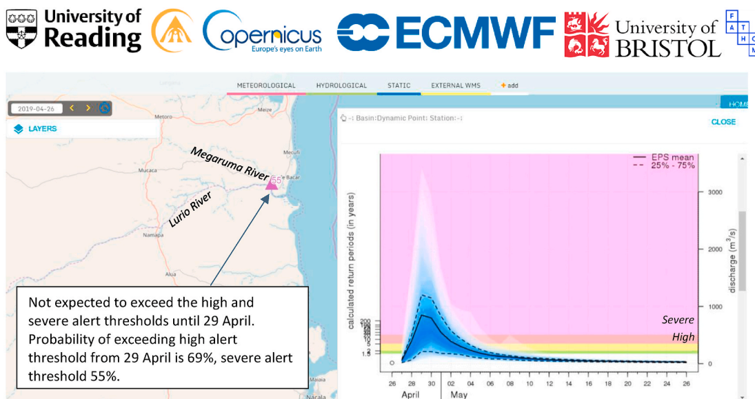
Figure 6 Forecast hydrograph for warning point (lat/lon -13.45/40.45) on the Megaruma River in the Cabo Delgado province of Mozambique. Source: GloFAS, www.globalfloods.eu . Forecast issued 26-04-2019 00 UTC. Note: the warning point appears to be located between the Megaruma and Lurio rivers, due to the grid used in GloFAS. This has been cross-checked with other information, and this warning point is confirmed to be for the Megaruma river.
