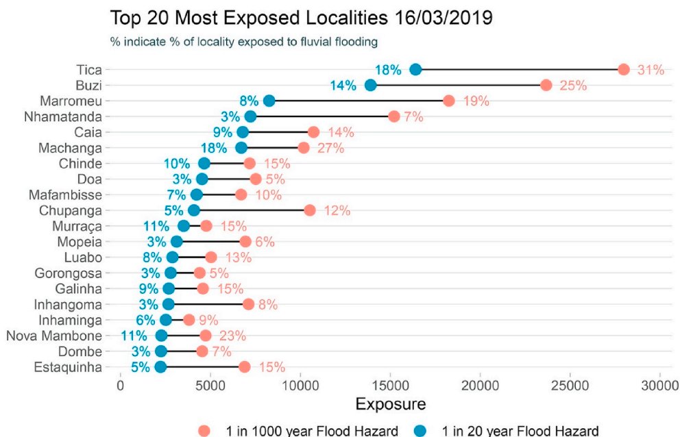
Fig. 9. Top 20 most exposed localities for Cyclone Idai on 16/03/2019. The blue circles indicate the exposure to the 20-year return period (5% AEP) flood inundation and red the exposure to the most extreme 1000-year (0.1% AEP) flood inundation. The percentage of the total locality population exposed to flooding is also shown. (For interpretation of the references to colour in this figure legend, the reader is referred to the Web version of this article.)
