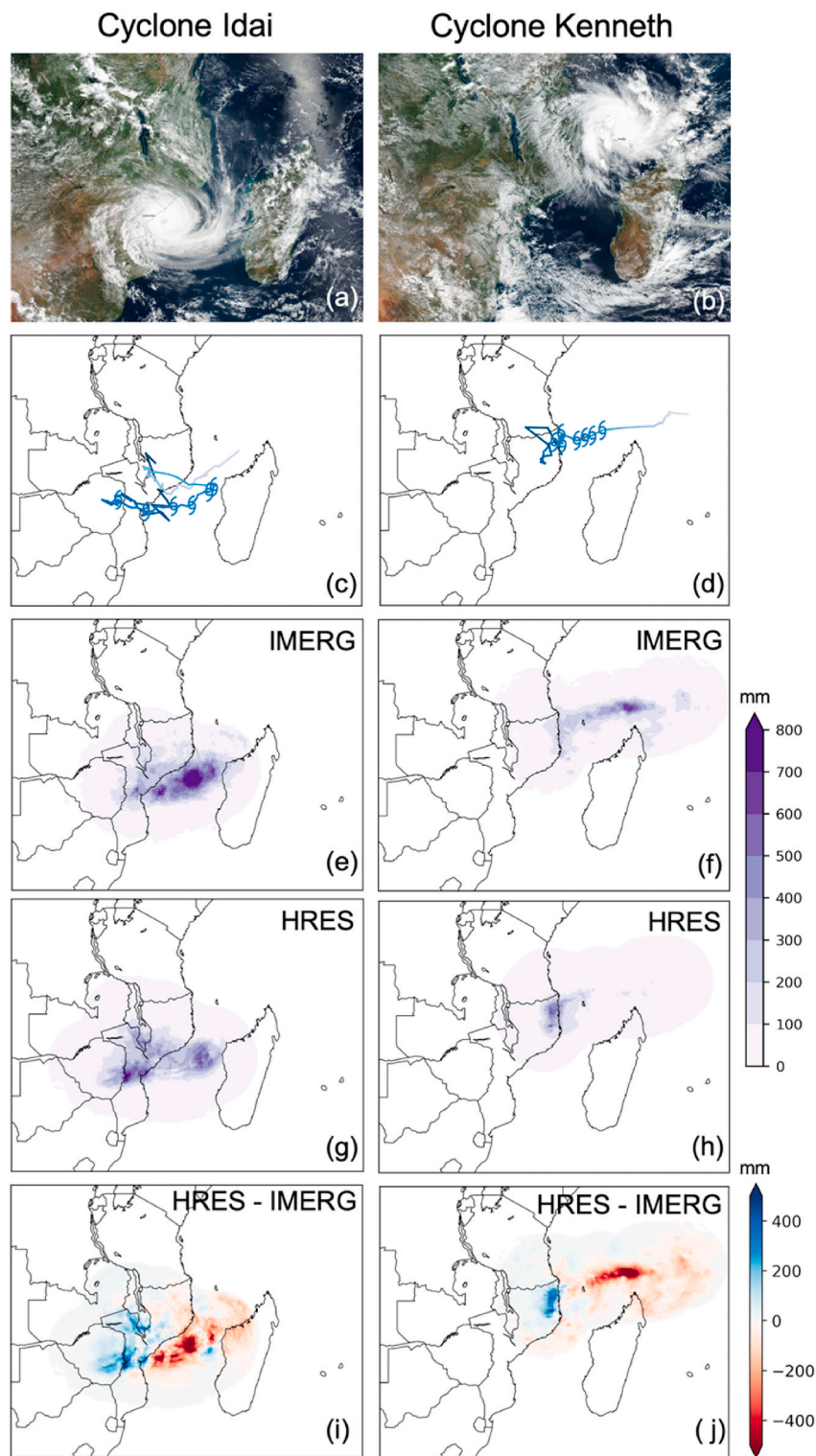
Fig. 4. Observed tracks and rainfall analysis for Cyclones Idai and Kenneth. The top panels show satellite images (NASA Worldview, 2019) of (a) Cyclone Idai, taken on 14th March 2019 and (b) Cyclone Kenneth, taken on 24th April 2019, followed by the tracks of (c) Cyclone Idai and (d) Cyclone Kenneth from genesis to dissipation, identified in the ECMWF operational analysis data using the methodology described in section 3.1. Tracks progress from light to dark shading, and cyclone symbols depict the portion of the track when the storms were classified as tropical cyclones. Total observed rainfall (mm) is shown for (e) Cyclone Idai, from 1 to 24 March 2019, and (f) Cyclone Kenneth, from 21st to 28th April 2019, using the IMERG satellite precipitation data (see section 3.1). Also shown is the total forecast rainfall (mm) from the ECMWF HRES forecasts at 1 day lead time , for (g) Cyclone Idai and (h) Cyclone Kenneth. This is the sum of all 24-h rainfall accumulations from forecasts produced 1 day ahead (for example, a forecast produced at 00UTC on 12th March for the 24-h total rainfall accumulation on 13th March) for the duration of each storm. Finally, the mean error of the total rainfall forecast (mm) of the ECMWF HRES forecasts at 1 day lead time is shown for (i) Cyclone Idai and (j) Cyclone Kenneth. Red indicates too little rainfall, and blue indicates too much rainfall in the forecasts. (For interpretation of the references to colour in this figure legend, the reader is referred to the Web version of this article.)
