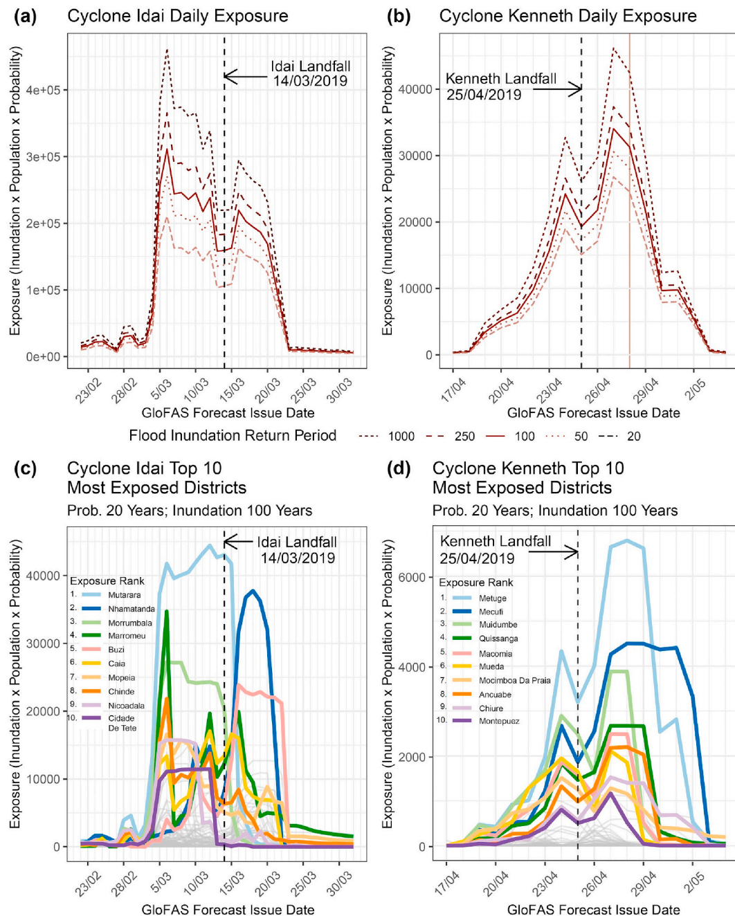
Fig. 8. Daily total exposure estimates for Mozambique for (a) Cyclone Idai and (b) Cyclone Kenneth, for five different flood inundation return periods (20, 50, 100, 250 and 1000-year return periods, equivalent to 5%, 2%, 1%, 0.4% and 0.1% AEPs, respectively, indicated by different line styles), and exposure per district for (c) Cyclone Idai and (d) Cyclone Kenneth. The ranking is based on the total number exposed during the period shown on the graph. The faded grey lines are other districts in Mozambique, outside of the 10 districts with the highest exposure. The exposure per district is calculated based on the severe flood level of GloFAS (20-year return period/5% AEP), the 100-year (1% AEP) inundation return period and the HRSL population dataset.
