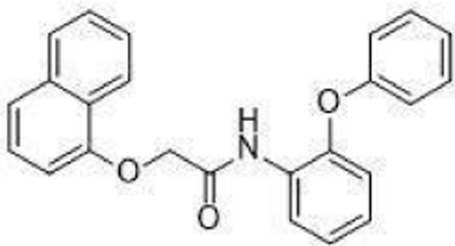
Fig. 1. Structure of GRA2, (2-(1-naphthyloxy)-N(2-phenoxyphenyl)acetamide).
