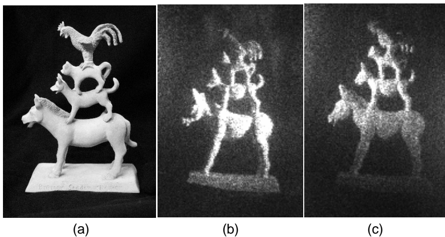
Figure 3. An example object captured: (a) photograph of the object, (b) a digital reconstruction from a hologram where the object was illuminated from a single direction, and (c) the improved results (fewer voids representing regions in shadow) by illuminating the object from two directions.
