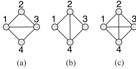
Figure 3.34: A single plaquette with (a) horizontal, (b) vertical and (c) both horizontal and vertical defects.
