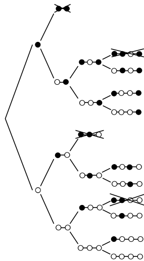
Figure 3.40: Tree representing configurations on a four site chain. Configurations that are crossed out break the nearest neighbour exclusion condition.
