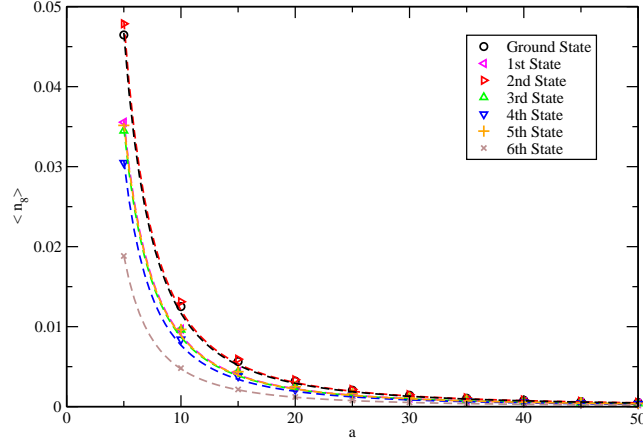
Figure 3.17: The one point function values at site 8 (one of the staggered sites) in the ground state and first excited states of the 18 site open staggered SUSY chain plotted against the staggering parameter a . The dashed lines are fits to the data with function f(a) = \frac{const.}{a^2} .
