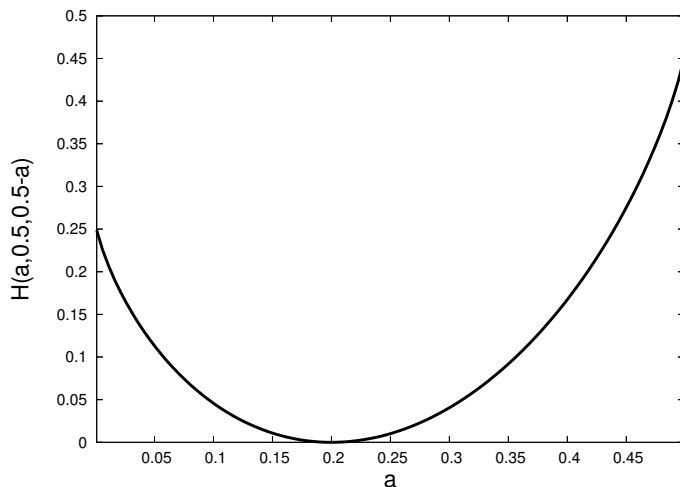
Figure 5.1: Empirical law rate function H(a, 0.5, 0.5 - a) for state selection in ITU-T P.59
