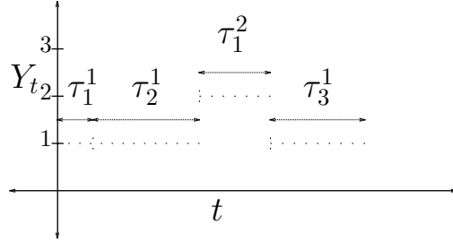
Figure 2.1: Example construction of the phase process \{Y_t\} .
