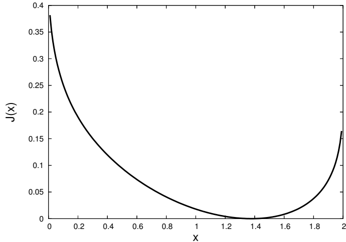
Figure 5.2: J_X(x) vs. x for a two way voice conversation based on ITU-T P.59
