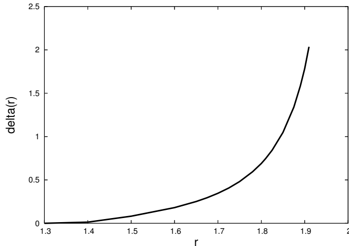
Figure 6.1: Rate of decay, \delta(r) , of the tail of the queue length distribution at a single server queue fed with ITU-T P.59 and serving at rate r , where \delta(r) = +\infty if r > 2
