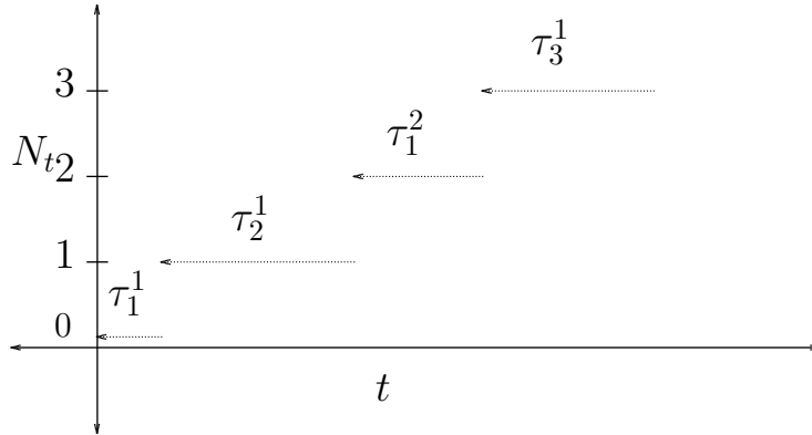
Figure 3.1: Example construction of the counting process \{N_t\} .
