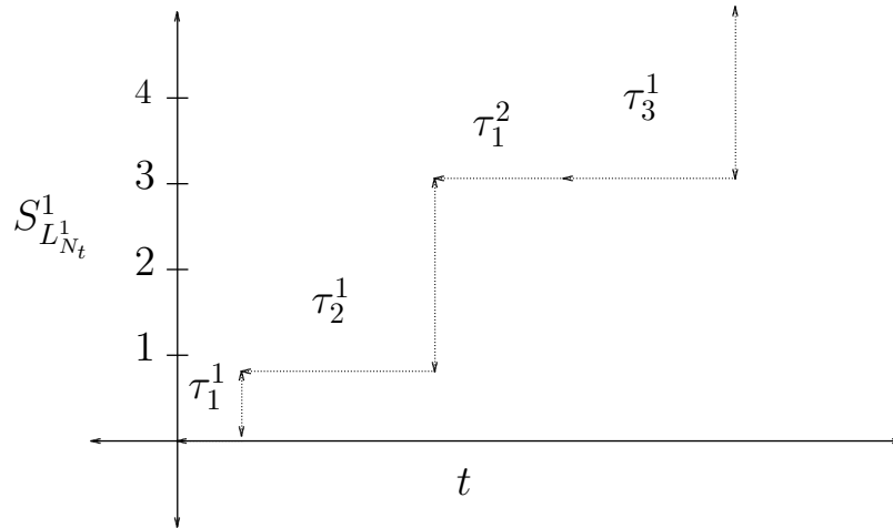
Figure 3.2: Example construction of the cumulative time spent in state 1 process \{S_{L_{N_t}}^1\} .
