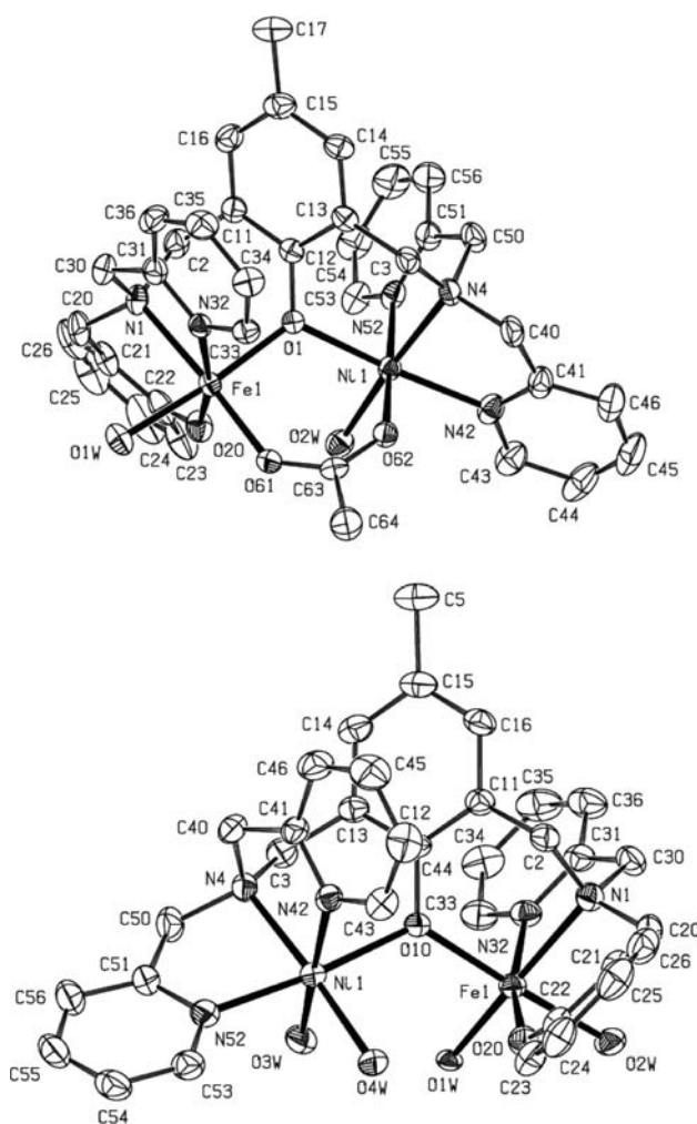
Fig. 4 Top: Crystal structure of [\text{Fe}(\text{III})\text{Ni}(\text{II})(\text{bpbmp})(\mu\text{-OAc})(\text{H}_2\text{O})_2](\text{ClO}_4)_2 \cdot 2\text{H}_2\text{O} ( 2 ). Bottom: Crystal structure of [\text{FeNi}(\text{bpbmp})(\text{OH})(\text{H}_2\text{O})_3](\text{ClO}_4)_2 \cdot 3\text{H}_2\text{O} ( 3 )
