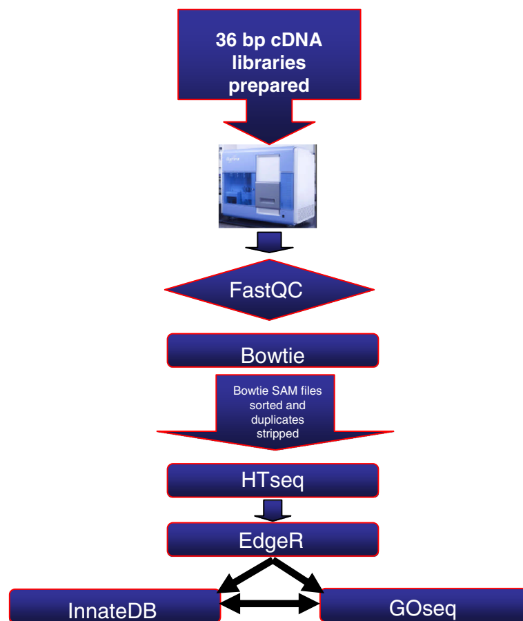
Figure 2 Bioinformatic pipeline employed in the analysis of RNA-seq data. Following sequencing on the GAIIi, FastQC was used to assess sequencing quality prior to aligning reads to the bovine genome with Bowtie. Counts were then assigned to each gene/exon with HTseq prior to the calculation of differential gene expression with EdgeR.
