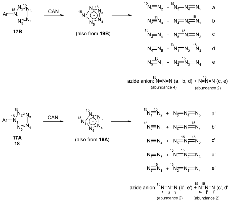
SCHEME 7. Expected Azide Anion ^{15}\text{N} Multiplicities and Intensities from Di- ^{15}\text{N} -Labeled Pentazoles (Ar = p -MeOC 6 H 4 - )
