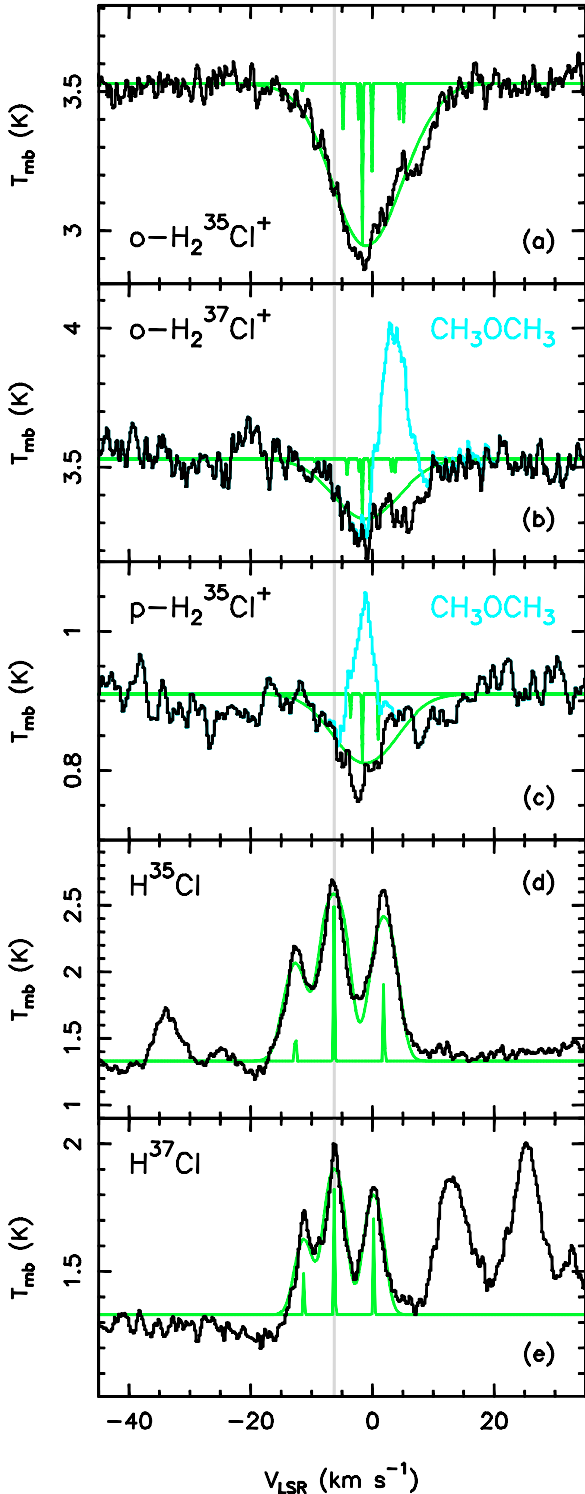
Fig. 1. Spectra of chlorine species in NGC 6334I: a) o\text{-H}_2^{35}\text{Cl}^+ 2_{12}\text{-}1_{01} ; b) o\text{-H}_2^{37}\text{Cl}^+ 2_{12}\text{-}1_{01} ; c) p\text{-H}_2^{35}\text{Cl}^+ 1_{11}\text{-}0_{00} ; d) \text{H}^{35}\text{Cl} 1\text{-}0 ; and e) \text{H}^{37}\text{Cl} 1\text{-}0 . The velocity scale corresponds to the strongest HFS components. Green lines show HFS fits and positions of the HFS components. The o\text{-H}_2^{37}\text{Cl}^+ and p\text{-H}_2^{35}\text{Cl}^+ lines are blended with dimethyl ether emission (light-blue lines in panels b) and c) .
