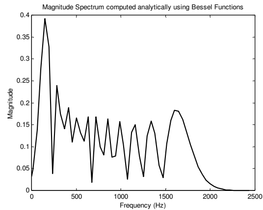
Figure 2: Magnitude spectrum of an Exponential FM signal using a Bessel Function Analysis.
