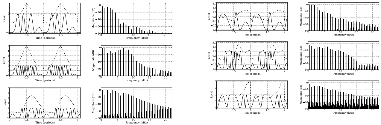
Figure 12: Lissajous audio-rate shape modulation of v vector component, f_m = f_0 , A_d = 1 and A_v = 3 (output, solid line; phase, dashed line) : (a) \omega_d = \omega_v and \theta = -\pi/2 (circular path); (b) \omega_v = 3\omega_d and \theta = -\pi/2 (three vertical rings); (c) \omega_d = \omega_v and \theta = 0.01 (nearly linear path)
