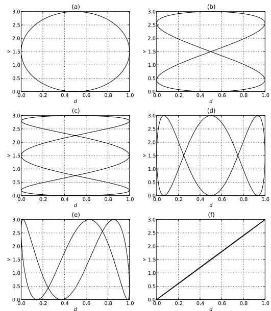
Figure 7: Lissajous modulation, with A_d = 1 and A_v = 3 : (a) \omega_d = \omega_v and \theta = \pi/2 ; (b) \omega_d = 2\omega_v and \theta = \pi/2 ; (c) \omega_d = 3\omega_v and \theta = \pi/2 ; (d) \omega_v = 3\omega_d and \theta = \pi/2 ; (e) \omega_v = 3\omega_d and \theta = \pi/4 ; (f) \omega_d = \omega_v and \theta = 0.01
