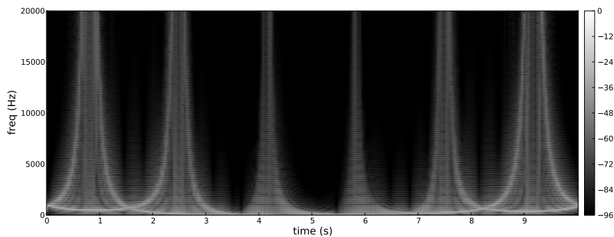
Figure 8: Spectrogram of VPS with Lissajous modulation, \omega_d = 3\omega_v , \theta = \pi/2 , A_d = 1 and A_v = 5
