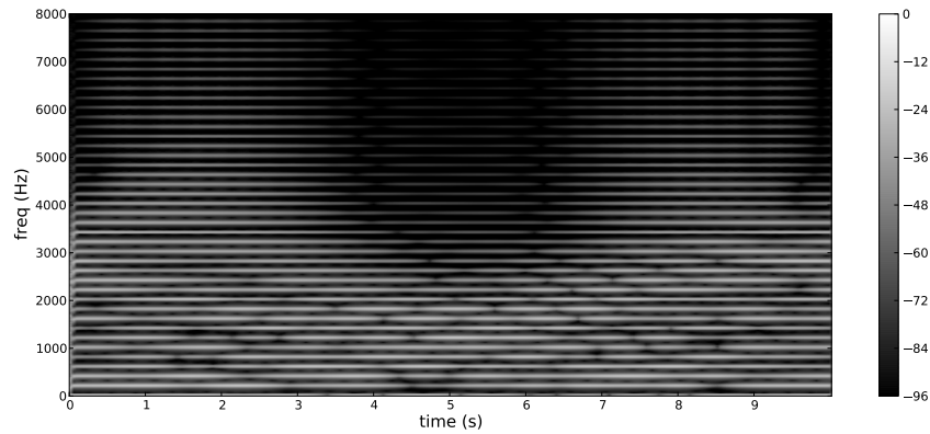
Figure 11: Spectrogram of an audio-rate modulated VPS timbre, d = 0.5 with v modulated by an inverted cosine, k = 5 , f_c = 500\text{Hz} , and f_m = f_c - 0.1 . The cyclically changing spectrum with a period of 10s is clearly displayed in this plot.
