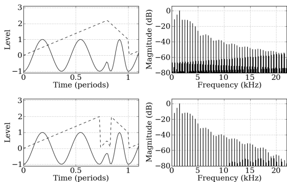
Figure 5: (a) trivial VPS timbre, and (b) its alias-suppressed form. p = (0.8, 2.2) .
