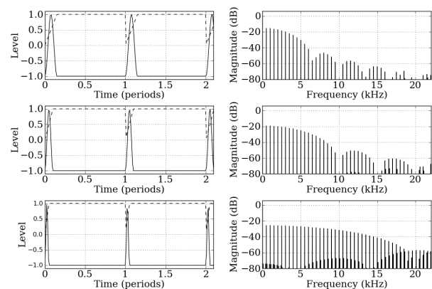
Figure 3: VPS pulse waveforms and spectra of three different widths, (a) p=(0.15,1) , (b) p=(0.1,1) , and (c) p=(0.05,1) .
