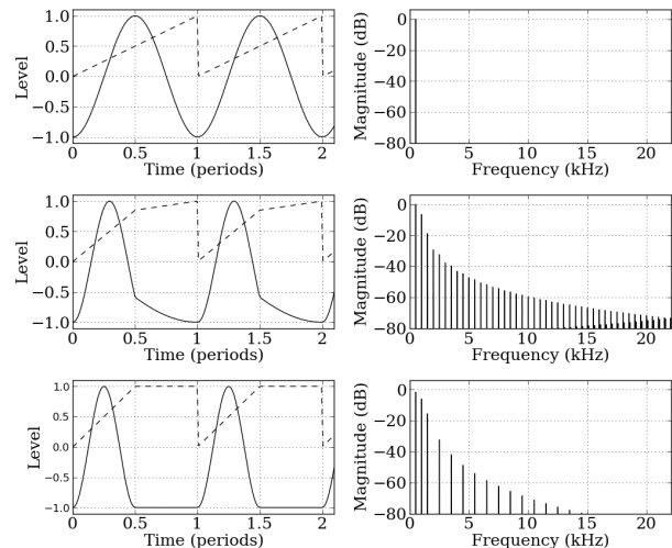
Figure 2: VPS waveforms and spectra of (a) p=(0.5,0.5) , (b) p=(0.5,0.85) , and (c) p=(0.5,1) . f_0 = 500\text{Hz} and f_s = 44100\text{ Hz} , as in all examples of this paper.
