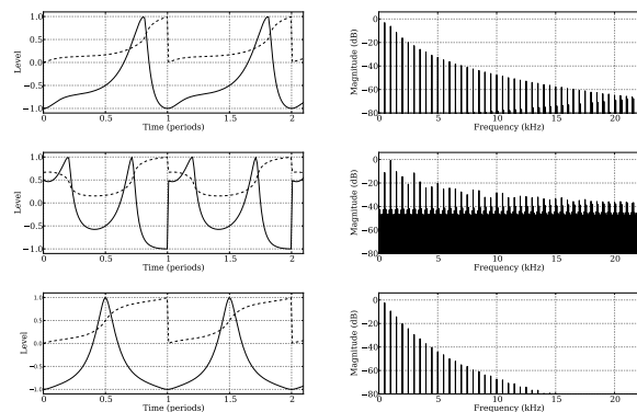
Figure 9: Audio-rate shape modulation of vector component d , f_m = f_0 (output, solid line; phase, dashed line): (a) Single-sided, inverted cosine modulator; (b) double-sided, inverted cosine modulator; and (c) double-sided, sine modulator
