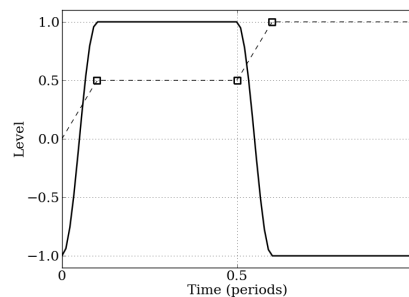
Figure 6: MVPS square-like waveform (thick) produced by a phase shaping function (dashed) with three inflection points at p_0 = (0.1, 0.5) , p_1 = (0.5, 0.5) and p_2 = (0.6, 1) .
