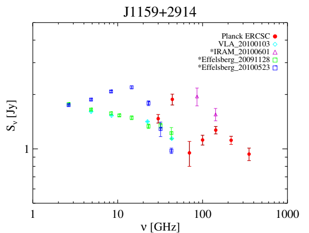
Fig. 11. The zig-zag shape spectrum of the strongly variable source J1159+2914. Asterisks identify epochs within 10 days from Planck observations at any of the LFI channels.
