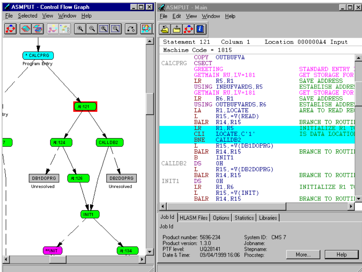
Figure 2 - Control Flow Graph (Corporation, 2010)
