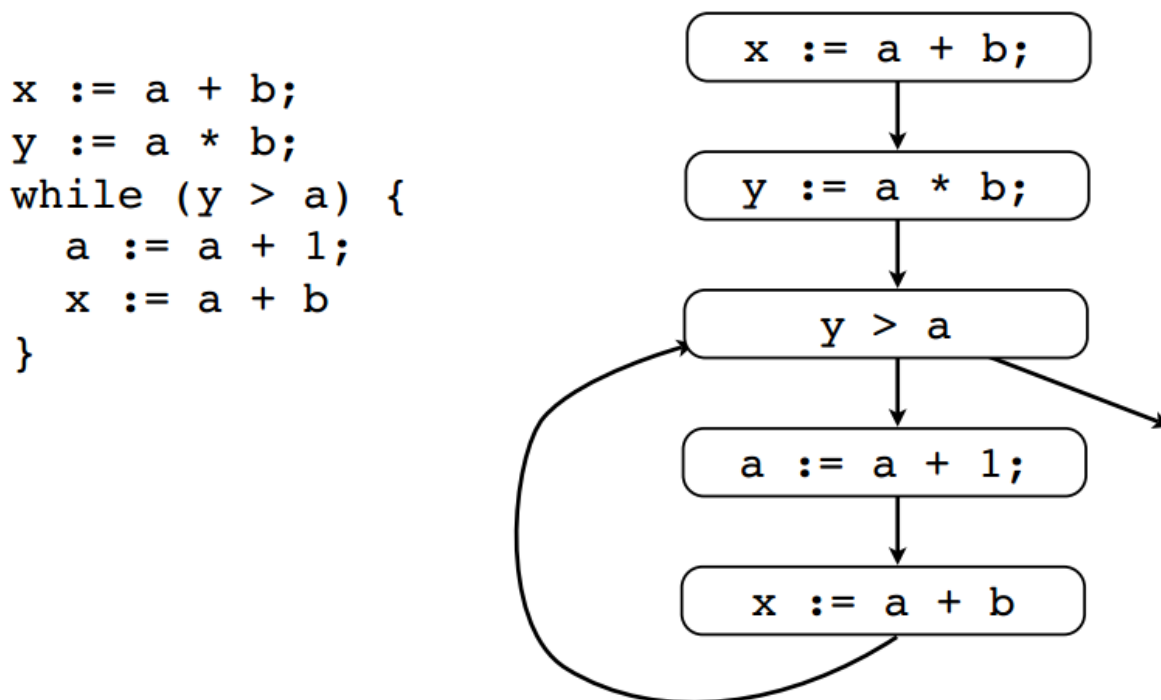
Figure 1 - Example of a Control Flow Graph (Foster, 2011)
