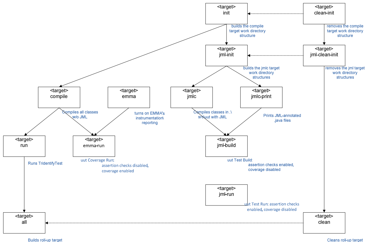
Figure 8 - Ant dependencies
