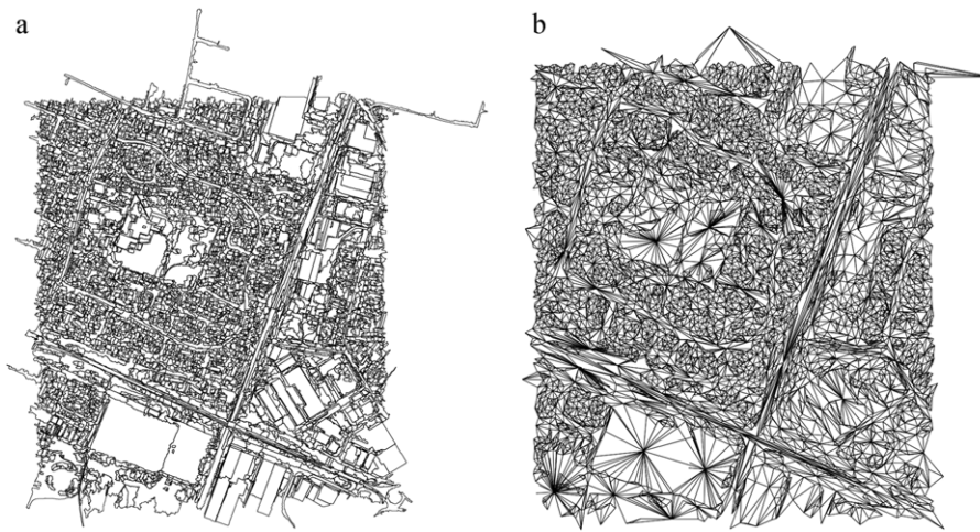
Fig. 1. (a) Land cover segments, (b) centroids of adjacent segments form network vertices joined by lines or graph edges.
