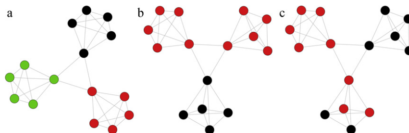
Fig. 2. Examples of modularity values for various different network communities: (a) with 3 communities, (b) and (c) with 2 communities. The Modularity scores are a) 0.576, b) 0.384 c) 0.253.
