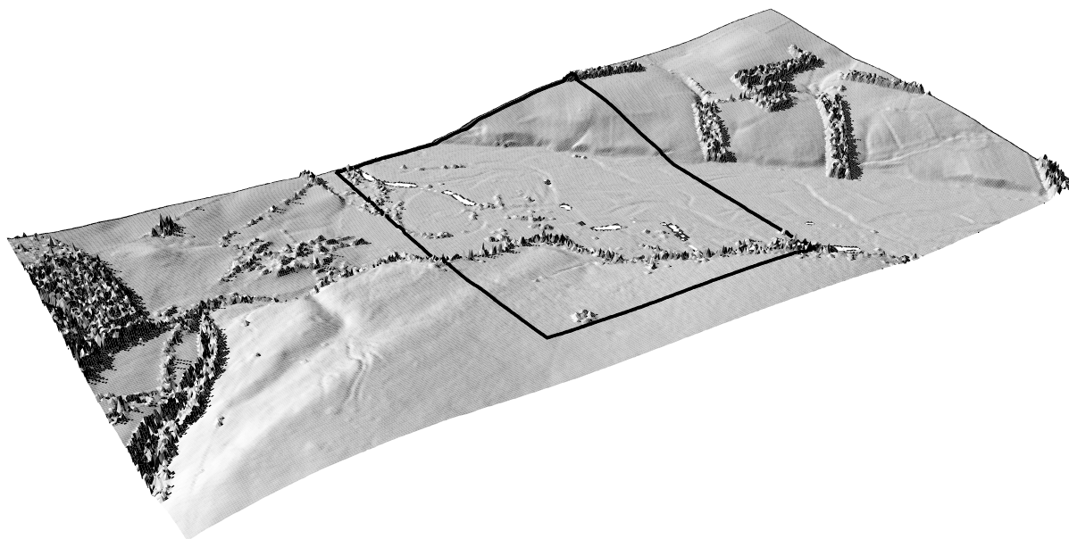
Figure 1. Perspective, viewed from the southwest, of the LiDAR elevation surface of a section of the River Coquet, showing the location of the study reach. The area shown is 2 km \times 1 km. Flow is from northwest to southeast
