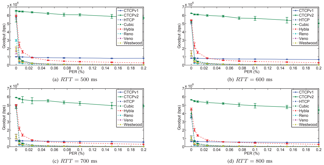
Figure 2: Comparison of TCP variants with varying PER and RTT with a link rate of 10 Mbps. Each bar shows the mean goodput, while the error bars show one standard deviation.
