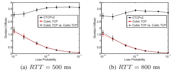
Figure 3: Goodput versus packet loss rate for (i) a Cubic TCP flow and CTCPv2 flow sharing a link (solid lines), and (ii) two Cubic TCP flows sharing a link (dashed line). The link rate is 5 Mbps and the error bars show one standard deviation.
