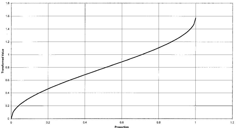
Figure 2. \arcsin[\sqrt{x}] transformation.
