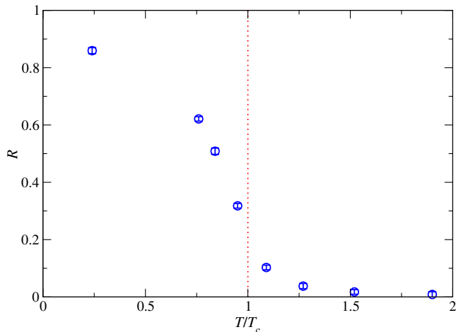
FIG. 4 (color online). Averaged ratio R in Eq. (11) as a function of T/T_c .
