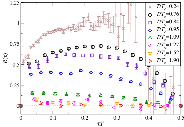
FIG. 3 (color online). Ratio R(\tau) in Eq. (10) as a function of \tau T .
