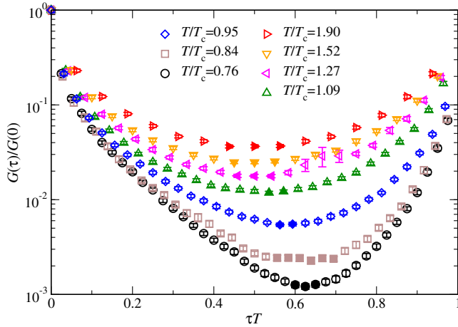
FIG. 1 (color online). Euclidean correlator G(\tau)/G(0) as a function of \tau T . At each temperature, the filled symbols indicate the minimum of the correlator, within the error.
