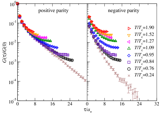
FIG. 2 (color online). Euclidean correlator G(\tau)/G(0) vs \tau/a_\tau for the positive-parity channel (left) and negative-parity channel, starting at the opposite side of the lattice (right).
