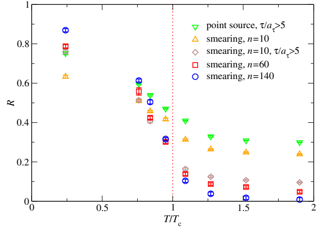
FIG. 5 (color online). As in Fig. 4, using point sources and different levels of smearing.
