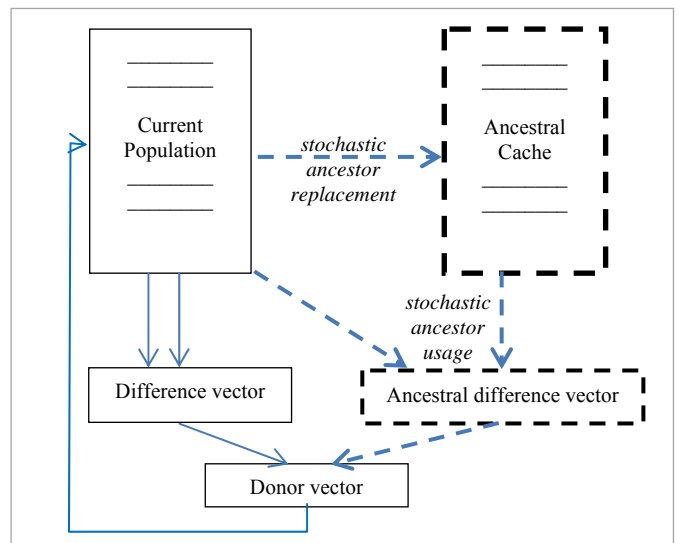
Fig. 1. Ancestral DE (AncDE) modifies DE by adding a cache of recent ancestors and the ability to derive difference vector between an agent from the population and one from the cache. The main modifications are highlighted by the dotted lines above. New ancestrally-based features have obvious parallels in (non-ancestral) normal DE.
