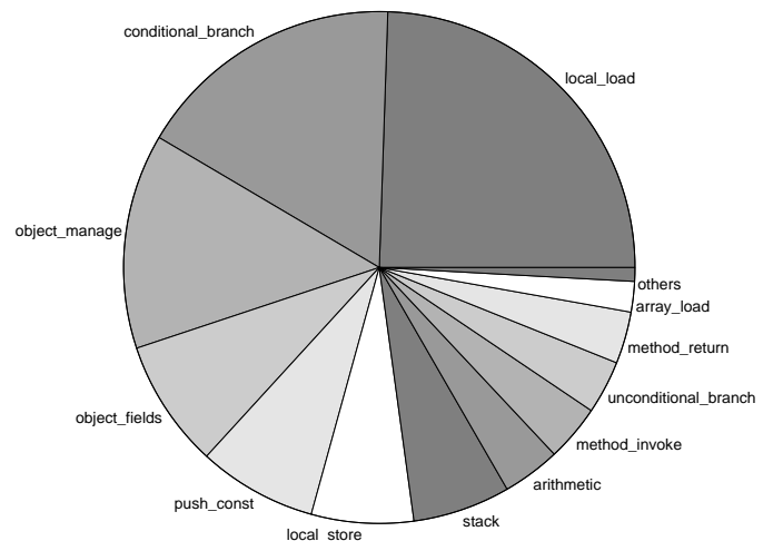
Figure 3: Total (API and Non-API) dynamic bytecode execution frequencies by category by the Eiffel programs studied when compiled using SmallEiffel no_check mode. Virtual Machine design, rather than the programming language used.
