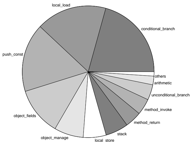
Figure 2: Total (API and Non-API) dynamic bytecode execution frequencies by category by the Eiffel programs studied when compiled using SmallEiffel all_check mode.
