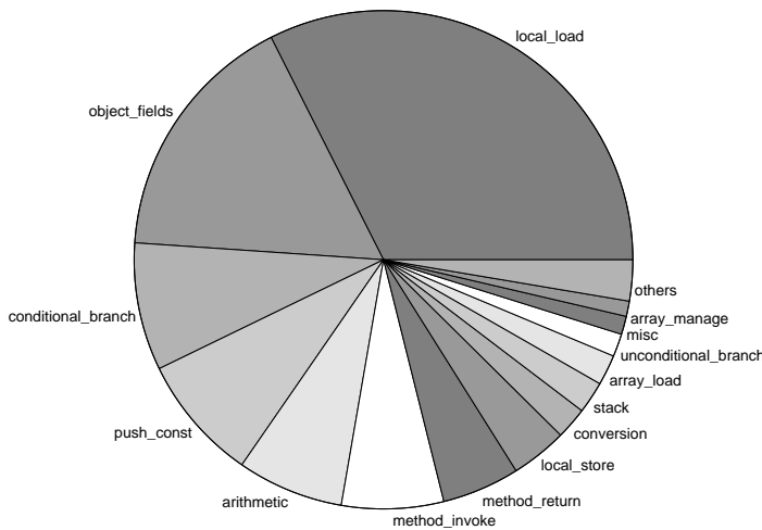
Figure 1: Total (API and Non-API) dynamic bytecode execution frequencies by category by the Java programs studied.
