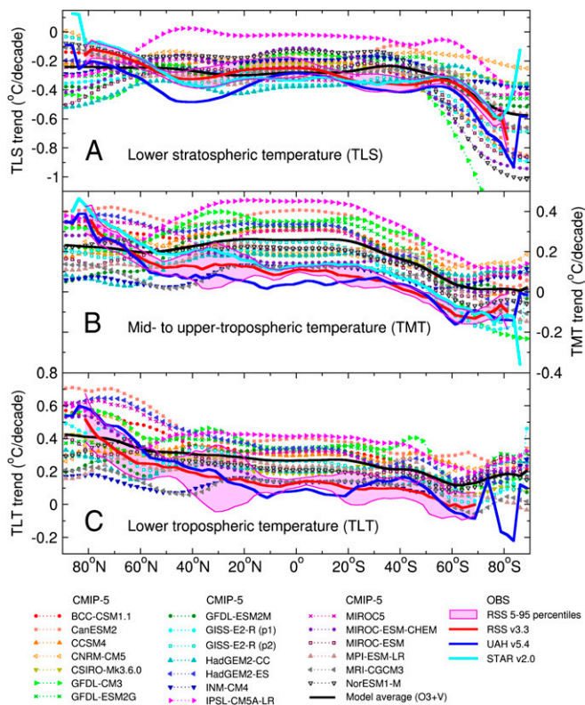
Fig. 3. Zonal mean trends in observed and synthetic (A) TLS, (B) TMT, and (C) TLT between 1979 and 2011. Observational results are from UAH, STAR, version 3.3 of the RSS dataset, and the 11 RSS 5–95 percentile realizations. Model synthetic MSU temperatures are from the spliced historical/RCP8.5 runs performed with 20 CMIP-5 models; only the first realization is shown for each model. The CMIP-5 multimodel averages are for the O3+V case. The 5th to 95th percentile range of the RSS results was computed as described in SI Appendix . The close agreement between RSS and UAH global mean TLT trends ( SI Appendix , Table S7) masks large differences in the latitudinal structure of each group’s TLT changes. The spatial coverage of the observational datasets differs at high latitudes and over areas of high elevation ( SI Appendix ). Note that STAR does not produce a TLT dataset.
