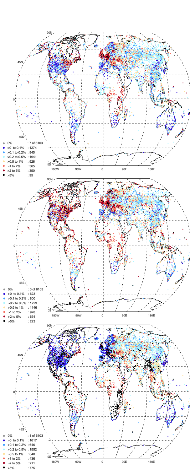
Fig. 20. Rejection rates by variable for each station. Top panel: temperature, Middle panel: dewpoint temperature, and Lower Panel: sea-level pressure. Different rejection rates are shown by different colours, and the key in each panel provides the total number of stations in each band.
