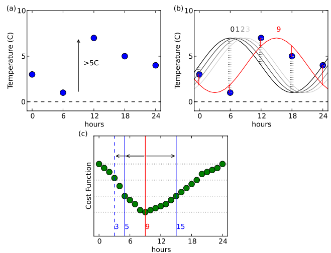
Fig. 5. Schematic for the diurnal cycle check. (a) An example time series for a given day. There are observations in more than 3 quartiles of the day and the diurnal range is more than 5 °C so the test will run. (b) A sine curve is fitted to the day observations. In this schematic case, the best fit that occurs has a 9-h shift. The cost function used to calculate the best fit is indicated by the dotted vertical lines. (c) The cost function distribution for each of the possible 24 offsets of the sine curve for this day. The terciles of the distribution are shown by horizontal black dotted lines. Where the cost function values enter the second tercile determines the uncertainty (vertical blue lines). The larger of the two differences (in this case 9 to 15 = 6 h) is chosen as the uncertainty. So if the climatological value is between 3 and 15 h, then this day does not have an anomalous diurnal cycle phase.
