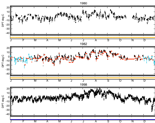
Fig. 9. Repeated streaks/unusual streak frequency check (test 8) example for composite station 724797-23176 (Milford, UT, USA; 38.44° N, 112.038° W, 1534 m), for dewpoint temperature in 1982, illustrating frequent short streaks. Red points show values removed by this test and blue points by other tests. The panel below each year shows whether the data in the composited station come from the named station (blue) or a matched station (orange). There is no change in source station in 1982, and so the compositing has not caused the streaks observed in 1982, but a different station is used in 1998 compared to the other two years.
