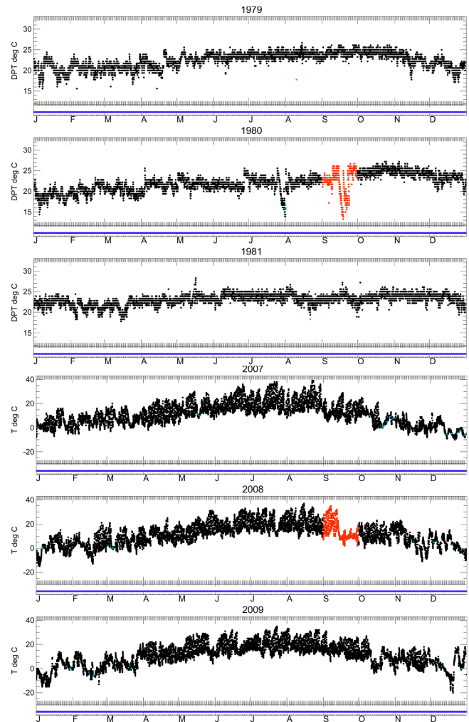
Fig. 13. Unusual variance check (test 13) for (top) 912180-99999 (13.57° N, 144.917° E, 162 m, Andersen Air Force Base, Guam) for dewpoint temperature and (bottom) 133530-99999 (43.82° N, 18.33° E, 511 m, Sarajevo, Bosnia-Herzegovina) for temperature. Red points show values removed by this test and blue points by other tests (none for the years and variables shown).
