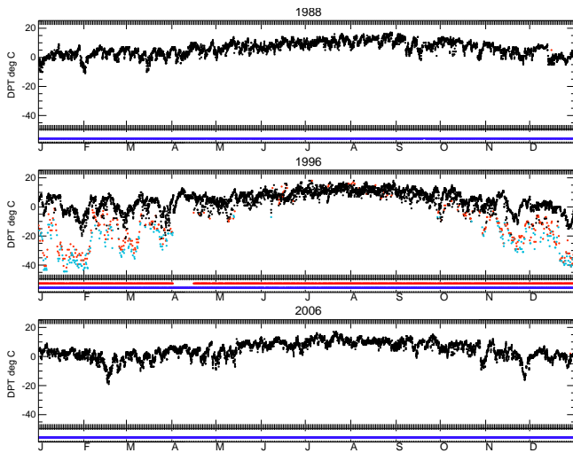
Fig. 12. Spike check (test 10) for composite station 718936-99999 (49.95° N, 125.267° W, 106 m, Campbell River, BC, Canada), for dewpoint temperature showing the removal of a ghost station. Red points show values removed by this test and blue points by other tests. The panel below each year shows whether the data in the composited station come from the named station (blue) or a matched station (red). In 1988 and 2006 a single station is used for the data, but in 1996 there is clearly a blend between two stations (718936-99999 and 712050-99999). In this case the compositing has caused the ghosting; however, both these stations are labelled in the ISD history file as Campbell River, with identical latitudes and longitudes. An earlier period of merger between these two stations did not lead to any ghosting effects.
