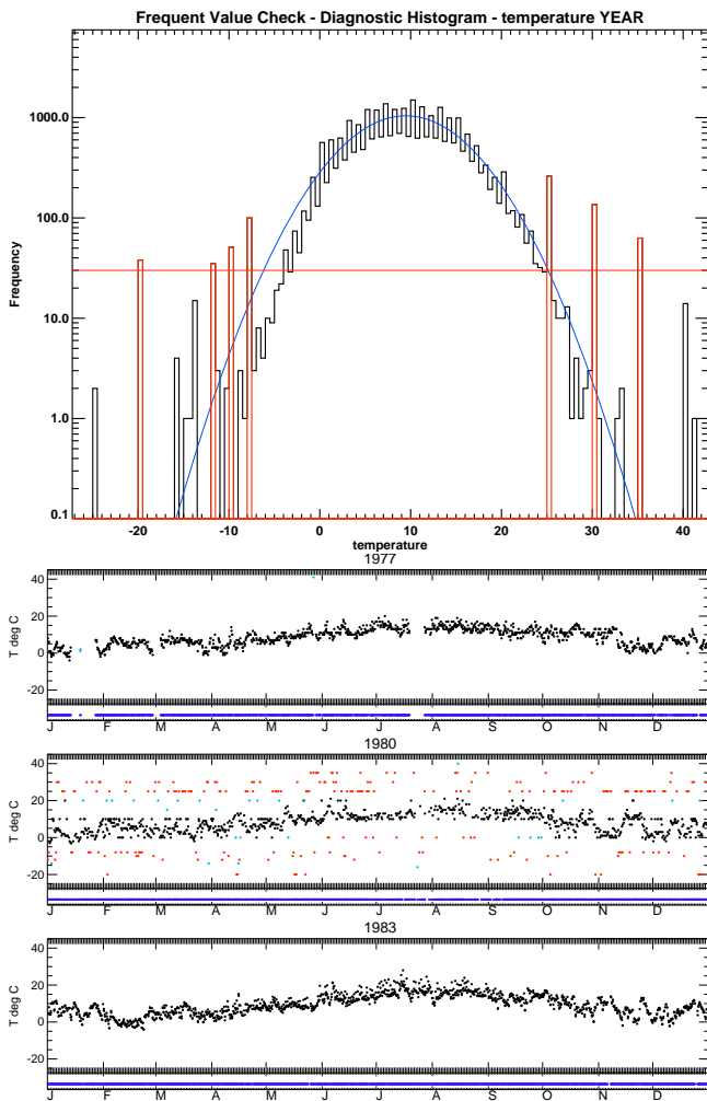
Fig. 4. Frequent value check (test 4) for station 037930-99999, Anvil Green, Kent, UK (51.22° N, 1.000° E, 140 m), showing temperature. Top: Histogram with logarithmic y-axis for entire station record showing the bins which have been identified as being likely frequent values. Bottom: red points show values removed by this test and blue points by other tests for the years 1977, 1980 and 1983. The panel below each year indicates which station the observations come from in the case of a composite (not relevant here but is relevant in other station plots so included in all).
