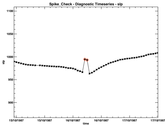
Fig. 16. Sea level pressure data from station 032450-99999 (Newcastle Weather Centre, 54.967° N, −1.617° W, 47 m) during mid-October 1987. The two observations that have triggered the spike check are clearly visible and are distinct from the rest of the data. Given their values (994.6 and 993.1 hPa), the two flagged observations are clearly separate from their adjacent ones (966.4 and 963.3 hPa). It is possible that a keying error in the SYNOP report led to 946 and 931 being reported, rather than 646 and 631. However, we make no attempt in this dataset to rescue flagged values.
