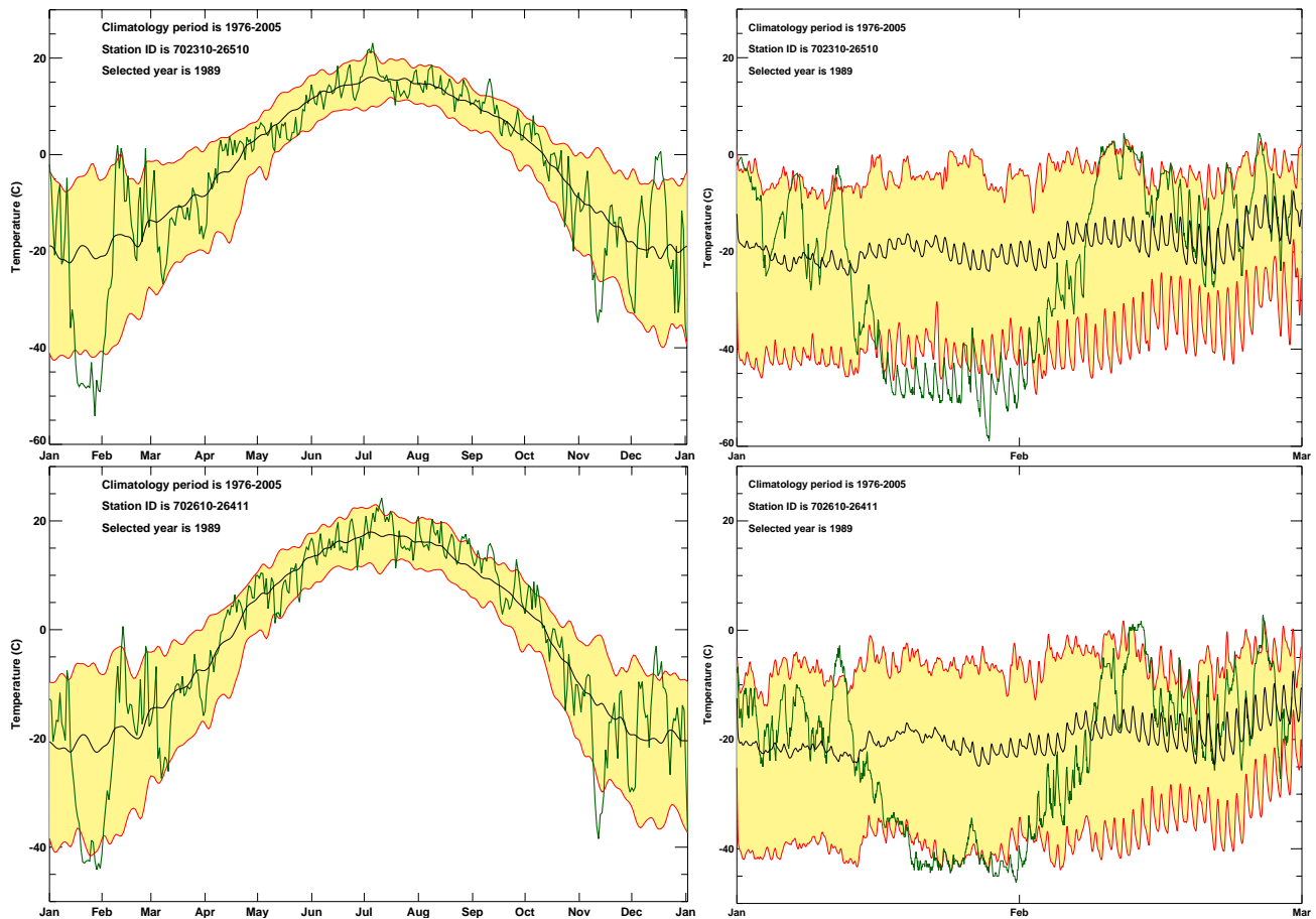
Fig. 18. Left: Alaskan daily mean temperature in 1989 (green curve) shown against the climatological daily average temperature (black line) and the 5th and 95th percentile region, red curves and yellow shading. The cold spell in late January is clearly visible. Right: similar plots, but showing the sub-daily resolution data for a two month period starting in January 1989. The climatology, 5th and 95th percentile lines have been smoothed using an 11-point binomial filter in all four plots. Top: McGrath (702310-99999, 62.95° N, 155.60° W, 103 m), bottom: Fairbanks (702610-26411, 64.82° N, 147.86° W, 138 m).
