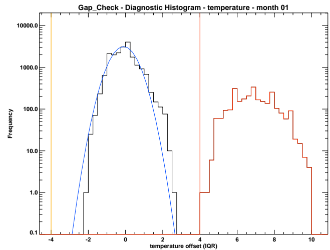
Fig. 8. Distribution of the observations from all Januaries in the station record for composite station 476960-43323, Yokosuka, Japan (35.58° N, 139.667° E, 530 m). The population highlighted in red is removed by the distributional gap check (test 6), as shown in Fig. 7. Note logarithmic y-axis.
