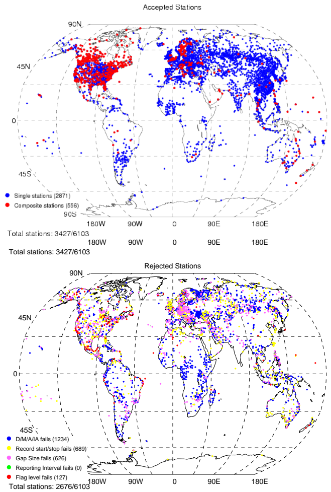
Fig. 21. The results of the final filtering to select climate quality stations. Top: the selected stations that pass the filtering, with red for composite stations (556/3427). Bottom: the rejected stations. Of these, 1234/2676 fail to meet the daily, monthly, annual or interannual requirements (D/M/A/IA); 689/2676 begin after 1980 or end before 2000; 626/2676 have a gap exceeding two years after the daily, monthly and annual completeness criteria have been applied; and 127 fail because one of the three main variables has a high proportion of flags.
