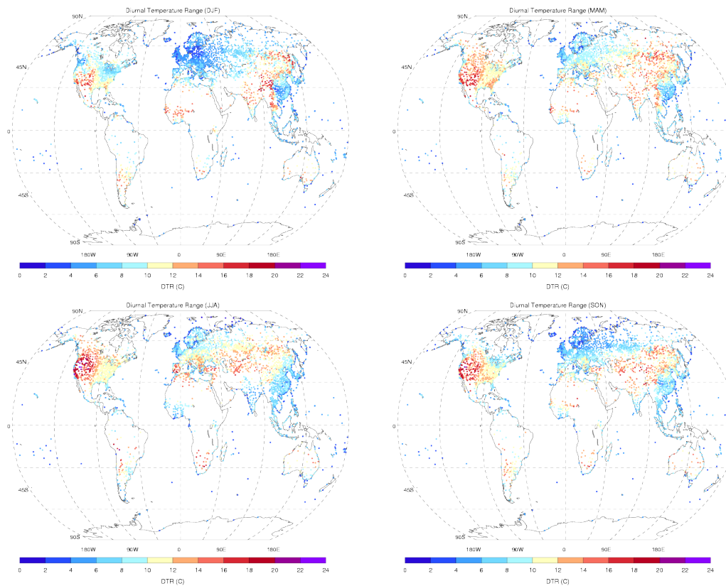
Fig. 22. The median diurnal temperature ranges recorded by each station (using the selected 3427 stations) for each of the four three-month seasons. Top-left for December-January-February, top-right for March-April-May, bottom-left for June-July-August and bottom-right for September-October-November.
