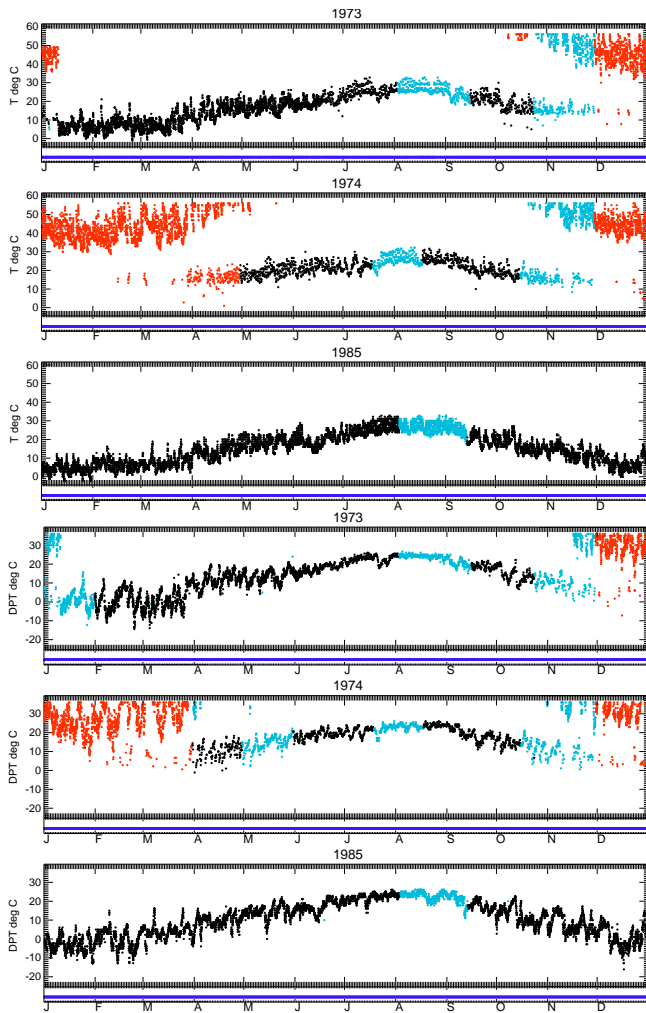
Fig. 7. Distributional gap check (test 6) example when comparing all of a given calendar month in the dataset for composite station 476960-43323, Yokosuka, Japan (35.58° N, 139.667° E, 530 m), for (top) temperature and (middle) dewpoint temperature for the years 1973, 1974 and 1985. Red points show values removed by this test and blue points by other tests (in this case, mainly the diurnal cycle check). The problem for this station affects both variables, but the tests are applied separately. There is no change in source station in any of the years, and so compositing has not caused the bad data quality of this station.
