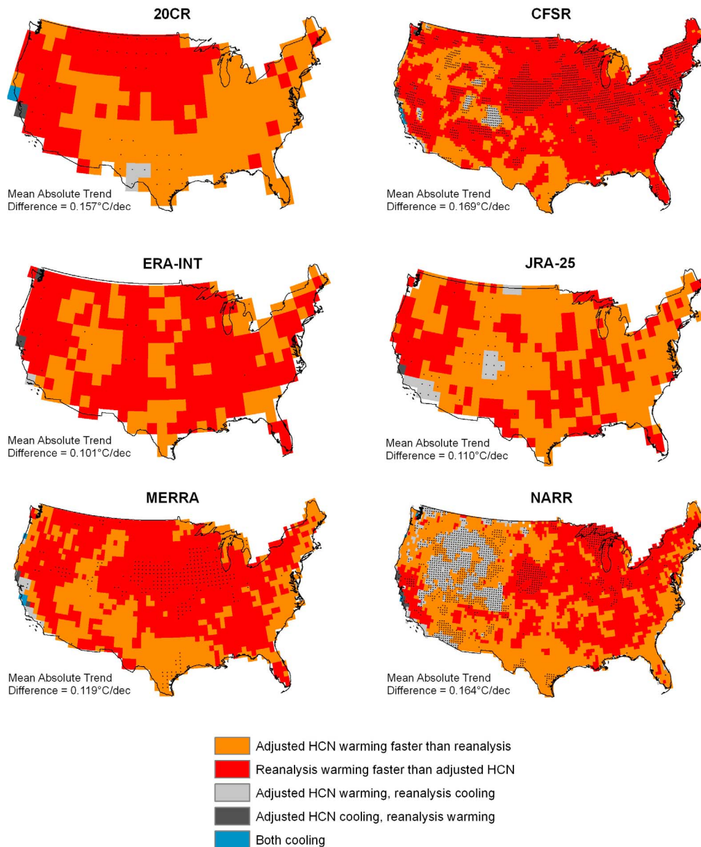
Figure 4. Categorical depiction of grid-box trends in mean annual temperature during the period 1979–2008. Stippled areas contain trend differences exceeding 0.25 \text{ }^{\circ}\text{C dec}^{-1} . The mean absolute trend difference is the area-weighted average of absolute trend differences across all grid boxes (i.e., the trend difference was computed for each grid box, then the sign was removed from that difference, then the unsigned grid-box differences were area-averaged into a single value for the conterminous United States).
