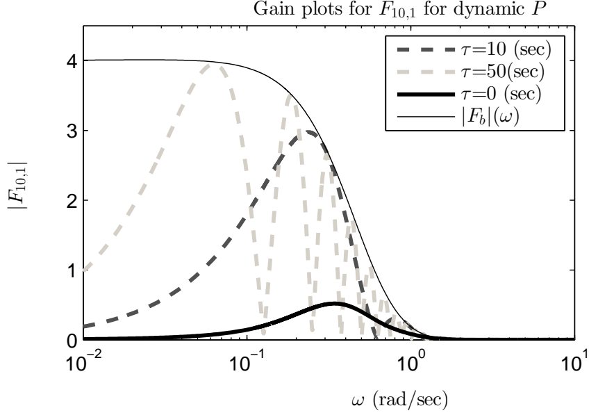
Figure 9: Magnitude plots of F_{10,1} for one-step string relay communications with dynamic P , n_r = 5 and \tau = \{0, 10, 50\} (sec). Solid thin line: |F_b|(\omega) .
