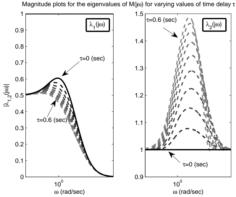
Figure 12: Magnitude plots of the eigenvalues \lambda_1(j\omega), \lambda_2(j\omega) of the matrix \mathcal{M}(j\omega) from the alternative algorithm for different magnitudes of time delay
