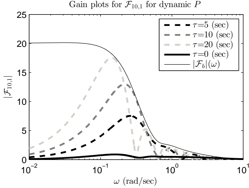
Figure 10: Magnitude plots of \mathcal{F}_{10,1} for one-step string relay communications with dynamic P, n_r = 5 and \tau = \{0, 5, 10, 20\} (sec). Solid thin line: |\mathcal{F}_b|(\omega) .
