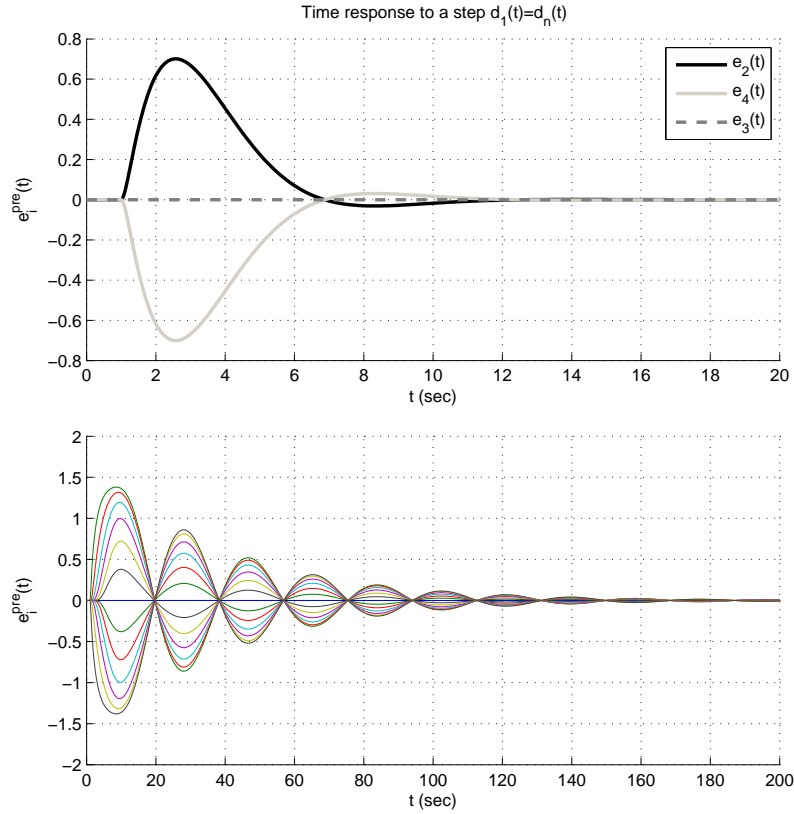
Figure 26: Time responses of the inter-vehicle spacings to a step in the front and rear vehicle. Symmetric static gains P = F = 0.5 for all s . Top: n = 4 . Bottom: n = 14 .
