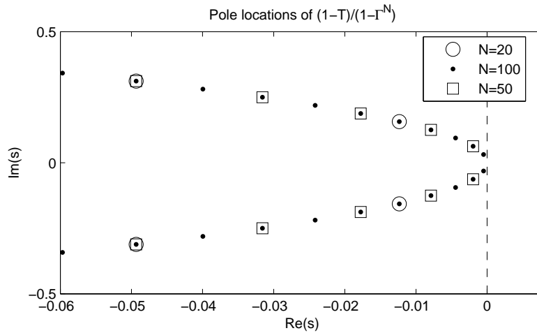
Figure 17: Pole locations for \frac{1-T}{1-T^n} with h = 2(\text{sec}) . Dashed line: Stability boundary. Circles: n=20 . Squares: n=50 . Dots: n=100 .
