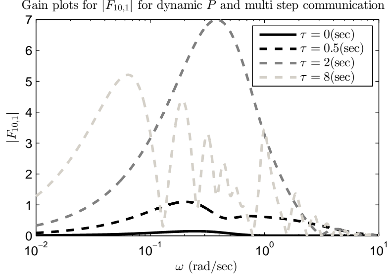
Figure 11: Magnitude plots of F_{10,1} for multi-step string relay communications with dynamic P , and \tau = \{0, 0.5, 2, 8\} (sec).
