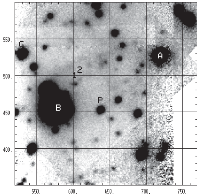
Fig. 2. B-band image of the core region of CTB 80. The image was made from the B-band observations listed in Table 1, and is equivalent to a total exposure of 16,456 seconds. The star identifications refer to those listed in Blair & Schild (1985). (1 pixel = 0''.23 , east is down and north is to the right)
