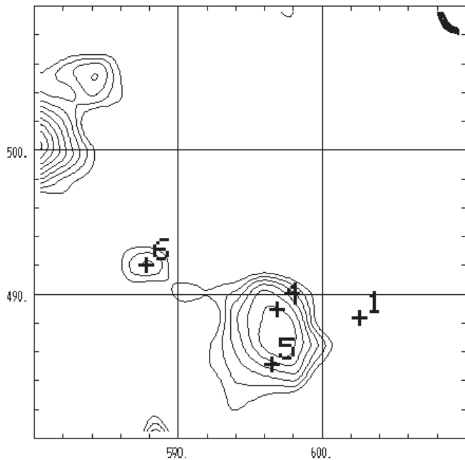
Fig. 4. Contour plot of the region surrounding candidate 1 in the V-band image of Fig. 1. The position of candidates discussed in the text are shown. The position of the radio pulsar (Foster et al. 1994) is close to candidate 4. (1 pixel = 0''.23 , east is down and north is to the right)
