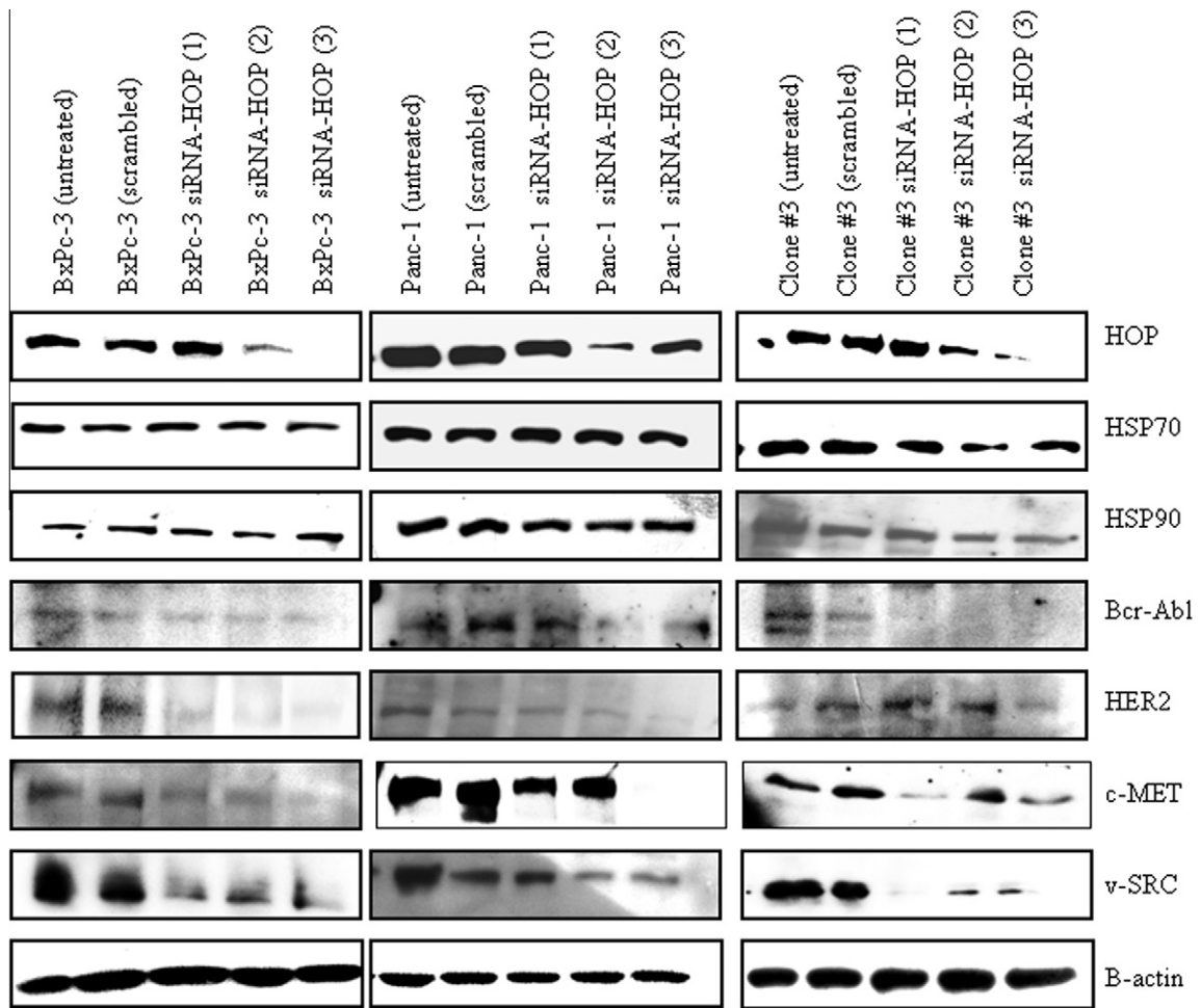
Fig. 5. Effect of Hop knockdown by siRNA on Hsp90 client proteins in BxPc-3, Panc-1 and Clone #3. Pancreatic cancer cells were transfected with three independent siRNAs against Hop and the scrambled control siRNA. A 72 h post transfection, the constitutive levels of Hop, Hsp90, Hsp70, HER2, Bcr-Abl, c-MET and v-Src were assayed by Western immunoblot.
