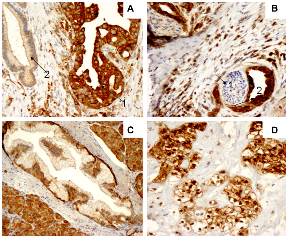
Fig. 6. Differential localisation of Hop in invasive pancreatic tumours. (A) PanIN grade 3 (arrow 1) displaying strong cytoplasmic Hop staining compared to PanIN grade 1 showing no Hop expression (arrow 2). (B) Perineural invasion in PDAC, cancer cells invading around the nerve (arrow 1) stained strongly for Hop (arrow 2). (C) PanIN grade 1 PDAC displaying sub-nuclear accumulation of Hop. (D) Invasive mucinous tumour displaying strong Hop complete membrane staining magnification 200 \times .
