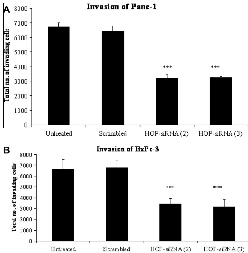
Fig. 2. Knockdown of Hop reduces the invasion of Panc-1 and BxPc-3 cells. A. Panc-1 and B. BxPc-3 cells were transfected with non-targeting scrambled siRNA (control siRNA) and two independent siRNA sequences against Hop. The total number of invading cells was determined by counting the number of cells per field in 10 random fields, at 200 \times magnification. The average number of cells per field was then multiplied by a factor of 140 (growth area of membrane/field area viewed at 200 \times magnification (calibrated using a microscope graticule)). Error bars represent the standard deviation of triplicate invasion assay experiments ( n = 3 ).
