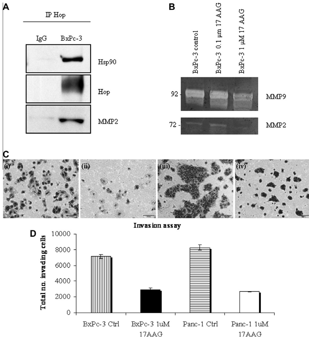
Fig. 4. Hop co-immunoprecipitates with Hsp90 and MMP-2. (A) Hop was immunoprecipitated from BxPc-3 conditioned media as described in materials and methods. Proteins were detected by MMP-2 and Hsp90 antibodies as indicated (right side of panel). (B) Effect of 17-AAG on pancreatic cancer. To validate Hop as an inhibitor of invasion in the Hsp90-complex, we used the Hsp90 pharmacological inhibitor 17-AAG and observed its effect on MMP-2 and MMP-9 expression. BxPc-3 cells were treated with 0.1 \mu M and 1 \mu M of 17-AAG for 24hrs under serum-free conditions. Conditioned medium was collected and MMP-2 and MMP-9 activities were analysed by gelatin zymography. (C) Representative invasion assay pictures of cells invaded through Boyden invasion chambers (8 \mu m pore size) coated with matrigel basement membrane matrix stained with 0.25% (w/v) crystal violet under control conditions and 24 h treatment with 1 \mu M 17-AAG in Panc-1 and BxPc-3 cells. Magnification 200 \times , scale bar 200 \mu m. (D) Invasion potential of Panc-1 and BxPc-3 cells treated with 1 \mu M 17-AAG as outlined in materials and methods. Graphs represented as the total number of invading cells, as determined by counting the number of cells per field in 10 random fields, at 200 \times magnification. The average number of cells per field was then multiplied by a factor of 140 (growth area of membrane/field area viewed at 200 \times magnification (calibrated using a microscope graticule)). Values are mean \pm standard deviation ( n = 3 ).
