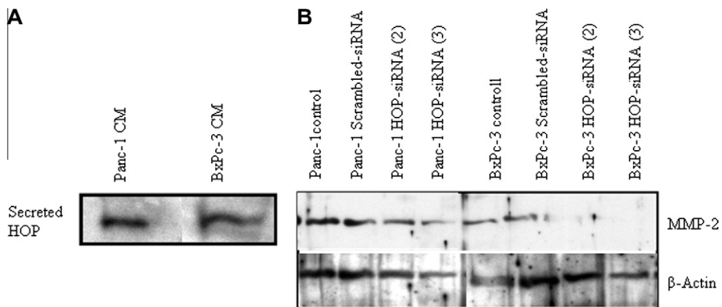
Fig. 3. Hop as an extracellular protein can disrupt MMP-2 expression. (A) Serum-free conditioned media from Panc-1 and BxPc-3 cells was collected, concentrated and immunoblotted for Hop. (B) Panc-1 and BxPc-3 cells transfected with Hop-siRNA (2) and (3) were immunoblotted for MMP-2.
