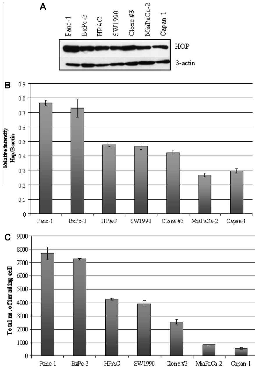
Fig. 1. Hop protein expression in human pancreatic cancer cells. (A) Representative Western immunoblot showing the expression of constitutive Hop in a panel of pancreatic cancer cell lines. Housekeeping gene \beta -actin was used as an internal control. (B) Densitometry analysis of Hop bands (normalised to \beta -actin). Error bars represent the standard deviation of triplicate experiments. (C) The invasive capacity of panel of cell lines. The total number of invading cells was determined by counting the number of cells per field in 10 random fields, at 200 \times magnification. The average number of cells per field was then multiplied by a factor of 140 (growth area of membrane/field area viewed at 200 \times magnification (calibrated using a microscope graticule)). Error bars represent the standard deviation of triplicate invasion assay experiments ( n = 3 ).
