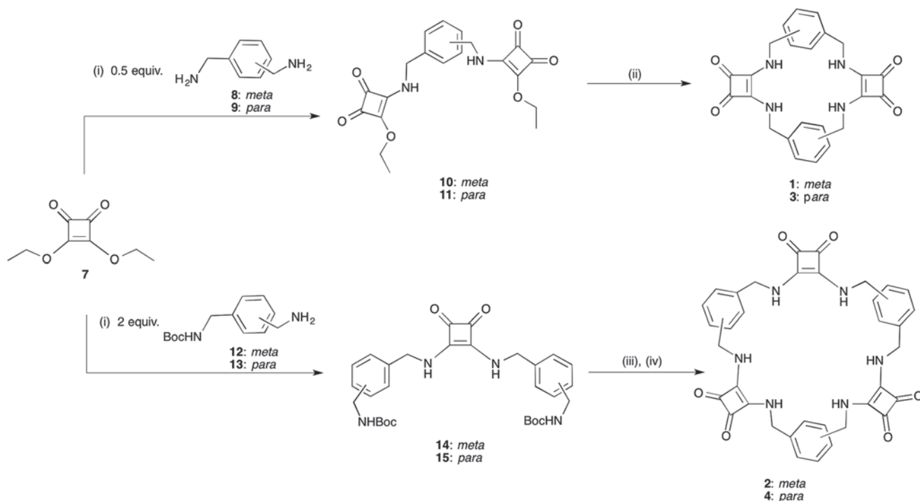
Scheme 1 Synthesis of the desired macrocyclic squaramide based receptor frameworks 1–4. Synthesis: (i) Et 3 N, EtOH; (ii) 1 equiv. 8 or 9, high dilution, Et 3 N, EtOH, heat. (iii) TFA/DCM (1 : 1); (iv) 1 equiv. 10 or 11, high dilution, Et 3 N, EtOH, heat.
