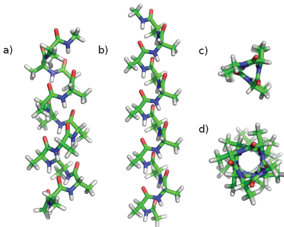
Fig. 4. Ideal helical conformations of Ala12: \alpha and 3_{10} helices are shown in panel a and b , respectively; while the lumen of the 3_{10} and \alpha helices is shown in panel c and d , respectively.
