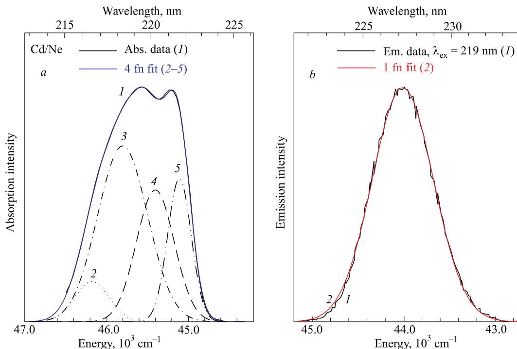
FIG. 9. Lineshape analyses of the Cd/Ne absorption (a) and emission (b) profiles recorded at 4.5 K. Four Gaussian functions were needed to provide an acceptable fit for the absorption profile while the emission profile was readily fit with a single Gaussian function. The three components in the blue portion of the absorption band are located at 46 177, 45 800 and 45 400 \text{cm}^{-1} (216.55, 218.34, 220.26 nm) with bandwidths of 499, 720, 544 \text{cm}^{-1} respectively. The red excitation component is centered at 45 105 \text{cm}^{-1} (221.70 nm) having a width is 340 \text{cm}^{-1} . The emission fit, shown on the right, yielded corresponding values of 44 008 \text{cm}^{-1} (227.23 nm) and a width of 790 \text{cm}^{-1} (b).
