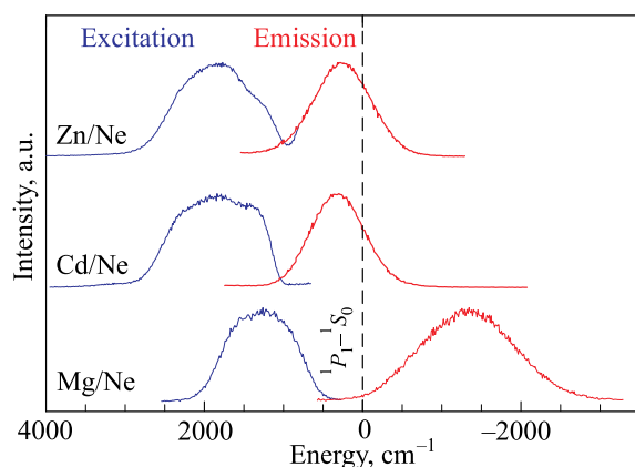
FIG. 10. An expanded presentation of the excitation/emission bands recorded for atomic Zn, Cd and Mg isolated in solid Ne highlighting the similarities of the Zn/Ne and Cd/Ne systems and the dissimilarity of Mg/Ne. For the purposes of comparison, all the features shown have been “zeroed” with respect to their respective np\ ^1P_1 - ns\ ^1S_0 gas phase transitions. Particularly evident is the similar behavior of the Zn/Ne and Cd/Ne systems whose bands are all to the blue of the gas phase atomic transition. In contrast, the matrix bands in Mg/Ne straddle the gas phase transition. Noteworthy also in Mg/Ne are the much greater bandwidth of the emission and simple excitation band which contrasts with the complex structures recorded in both Zn/Ne and Cd/Ne.
