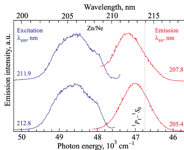
FIG. 4. A summary plot of all the excitation and emission features recorded at a temperature of 4.1 K for the 4s^14p^1\ ^1P_1-4s^2\ ^1S_0 transition of atomic Zn isolated in solid Ne. The lower panel denotes excitation and emission recorded from the dominant excitation feature, while the upper panel shows the luminescence recorded for the weaker red-shoulder in the excitation profile. The location of the ^1P_1-^1S_0 transition of atomic Zn in the gas phase is depicted by the vertical dotted line.
