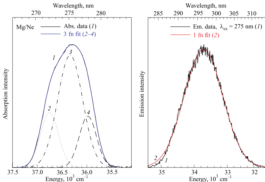
FIG. 7. Lineshape analyses of the Mg/Ne absorption and emission profiles done with Gaussian functions to resolve the components present. The absorption band consists of only three components located at 36\,755 , 36\,336 and 35\,979\text{ cm}^{-1} ( 272.07 , 275.21 , 277.94\text{ nm} ) with bandwidths of 429 , 595 , 411\text{ cm}^{-1} respectively. The emission fit, shown on the right, yielded corresponding values of 33\,718\text{ cm}^{-1} ( 296.57\text{ nm} ) and a width of 1380\text{ cm}^{-1} .
