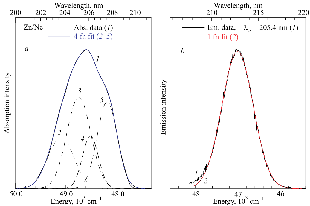
FIG. 5. Lineshape analyses of the absorption (a) and emission (b) spectra of Zn/Ne. Four Gaussian functions were required to provide a reasonable fit to the absorption profiles while only one is needed to fit the emission. The three features extracted in the blue absorption profile are located at 49 095, 48 740 and 48 509 \text{cm}^{-1} (203.68, 205.17 and 206.15 nm) with bandwidths of 600, 561 and 375 \text{cm}^{-1} respectively. The red excitation component is centered at 48 175 \text{cm}^{-1} (207.57 nm) having a width of 472 \text{cm}^{-1} . The quoted bandwidths are all fwhm values calculated as \Delta = s^* \sqrt{8 \ln(2)} where s is the variance in the fitted Gaussian function, G(x) = a \exp[-(x - m)^2 / (2s^2)] . A fit of the emission yielded a band centered at 47 006 \text{cm}^{-1} (212.73 nm) and a width of 872 \text{cm}^{-1} .
