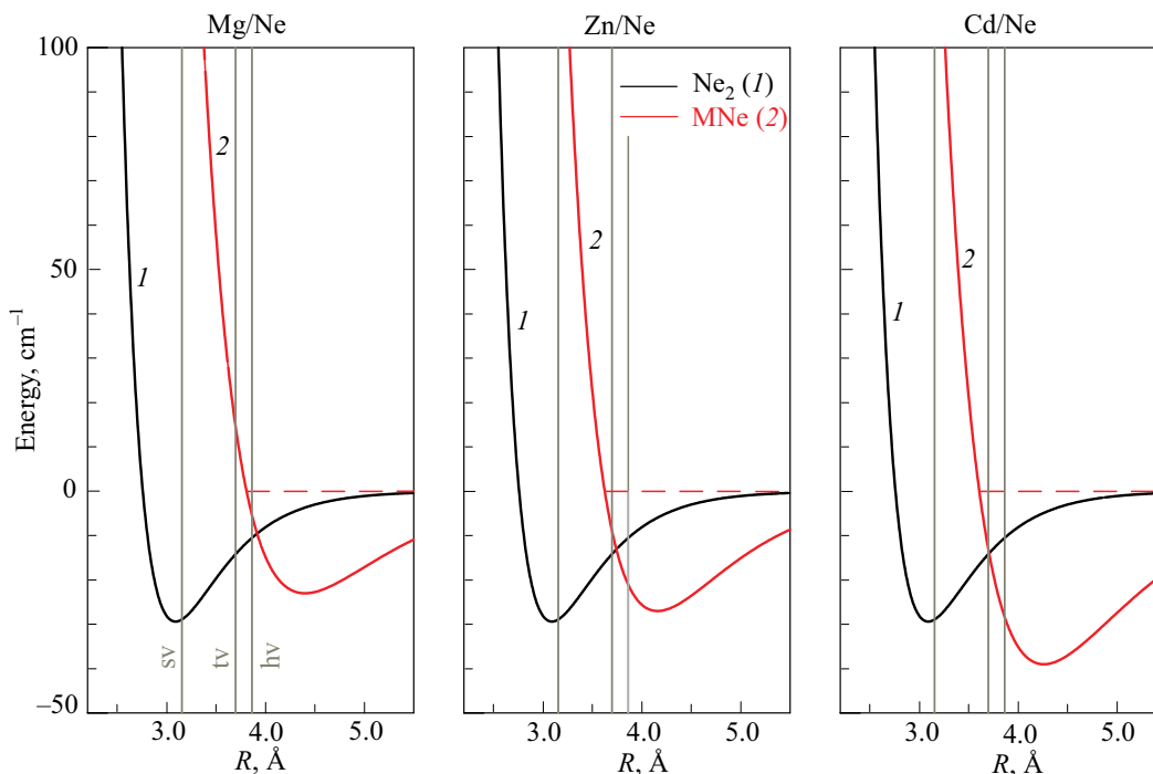
FIG. 11. A comparison of the potential energy curve of Ne dimer with the ground state X^1\Sigma state potentials for the diatomics Zn · Ne, Mg · Ne and Cd · Ne. The curves shown were generated with the data provided in Table 2. It is immediately evident that the bond lengths of the metal-neon diatomics are much greater than Ne dimer, an indication that substitutional site occupancy will be improbable for all three metal atoms in solid Ne. The size of this single vacancy (sv) site and the larger tetra-vacancy (tv) and hexa-vacancy (hv) sites are compared with the M · Ne potentials. This comparison reveals that the two larger sites have M–Ne distances on the bound portion of the Zn · Ne and Cd · Ne potentials, while only the largest hv site is in the bound portion of the Mg · Ne X^1\Sigma state potential.
