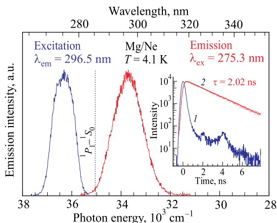
FIG. 6. Excitation and emission spectra recorded at 4.1 K in the Mg/Ne system after annealing to 8 K. The location of the Mg atom gas phase 3s^1 3p^1 \ ^1P_1 - 3s^2 \ ^1S_0 transition is represented by the vertical dotted line. Shown inset is a semi-log plot of the 296.5 nm emission (red dots) generated from excitation at 275 nm. The blue trace (1) centered at t = 0 is the temporal profile of the synchrotron radiation pulse. A single exponential fit of the decay curve, depicted by the solid red line (2), reveals a decay time of 2.02 ns.
