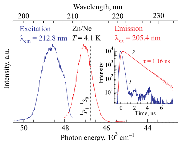
FIG. 3. Excitation and emission spectra recorded at 4.1 K in the Zn/Ne system after annealing to 8 K. As indicated, both excitation and emission are located to the blue of the gas phase atomic Zn 4s^14p^1\ ^1P_1-4s^2\ ^1S_0 transition, represented by the vertical dotted line. The inset shows a semi-log plot of the 213 nm emission decay curve, depicted by red dots, recorded with the TCSPC technique and generated from excitation at 205 nm. The blue curve (1) centered at t=0 is the temporal profile of the synchrotron radiation pulse. A single exponential function fit of the emission decay curve is depicted by the solid red line (2), yielding a lifetime of 1.16 ns.
