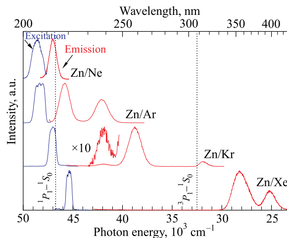
FIG. 12. A summary of the excitation and emission spectra recorded at 4.5 K for Zn atoms isolated in the solid rare gases. The Zn/RG samples were annealed to 8.9, 33, 45 and 65 K for Ne, Ar, Kr and Xe, respectively. The atomic Zn 4p^1P_1-4s^1S_0 and 4p^3P_1-4s^1S_0 gas phase transitions are identified by the vertical dotted line for comparison.
