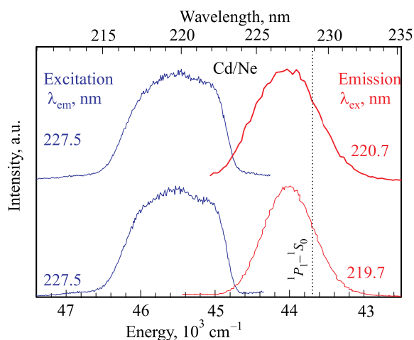
FIG. 8. A composite plot of the two excitation and emission features that arise for the Cd/Ne 5s^1 5p^1\ ^1P_1-5s^2\ ^1S_0 transition, recorded at a temperature of 4.5\text{ K} . The lower panel denotes emission recorded from the dominant feature in the excitation profile. The Cd gas phase ^1P_1-^1S_0 transition is portrayed by the dotted line.
