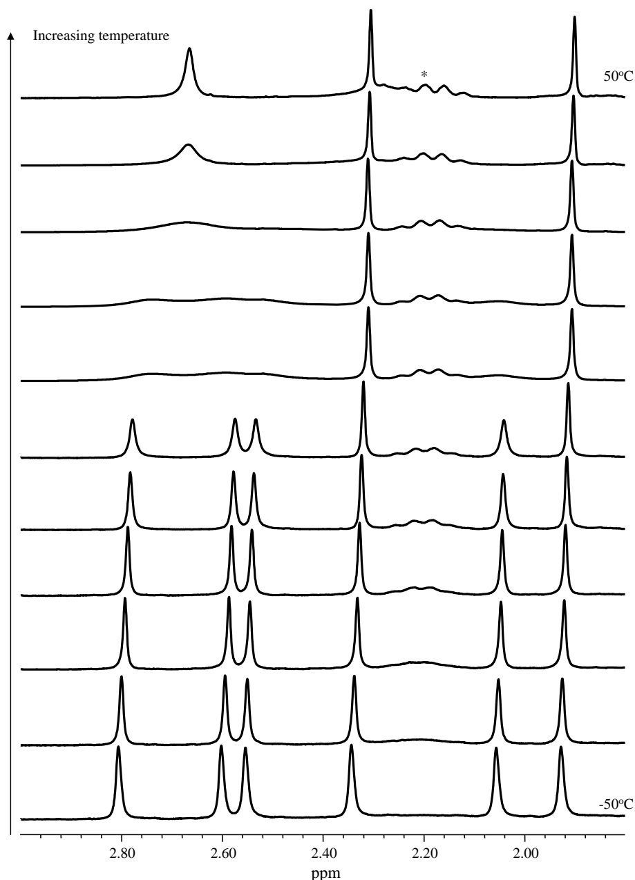
Fig. 4. ^1\text{H} NMR signals for the methyl groups on the mesitylene rings of 2 in \text{CDCl}_3 recorded as a function of temperature at 10^\circ\text{C} intervals. *Signals due to cyclohexyl groups on the phosphine ligand.
