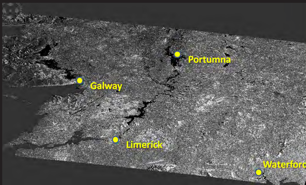
📡 An SAR image of parts of Munster/Connaught and the Shannon River. Strong returns are bright, whereas weak returns, such as water, are dark.
