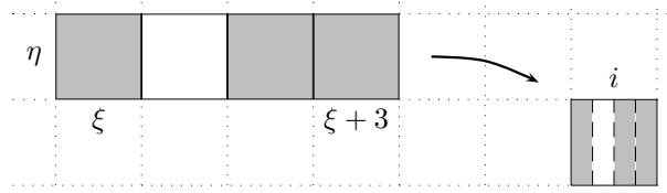
Fig. 2. Illustration of the instruction i \leftarrow [\xi, \xi + 3, \eta, \eta] that copies four images to a single image that is denoted i .
