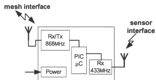
Figure 2: Mesh node
