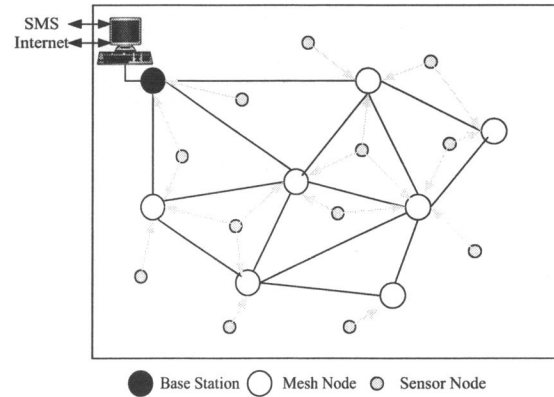
Figure 1: System Topology
