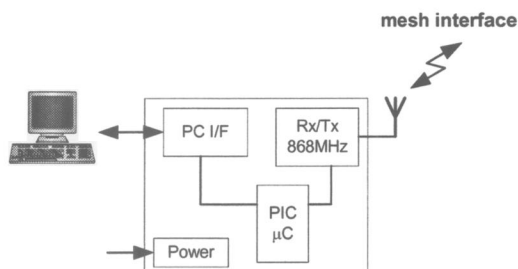
Figure 4: Base Station
