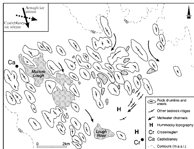
Fig. 4. Morphology of bedforms in the Crossmaglen area.
