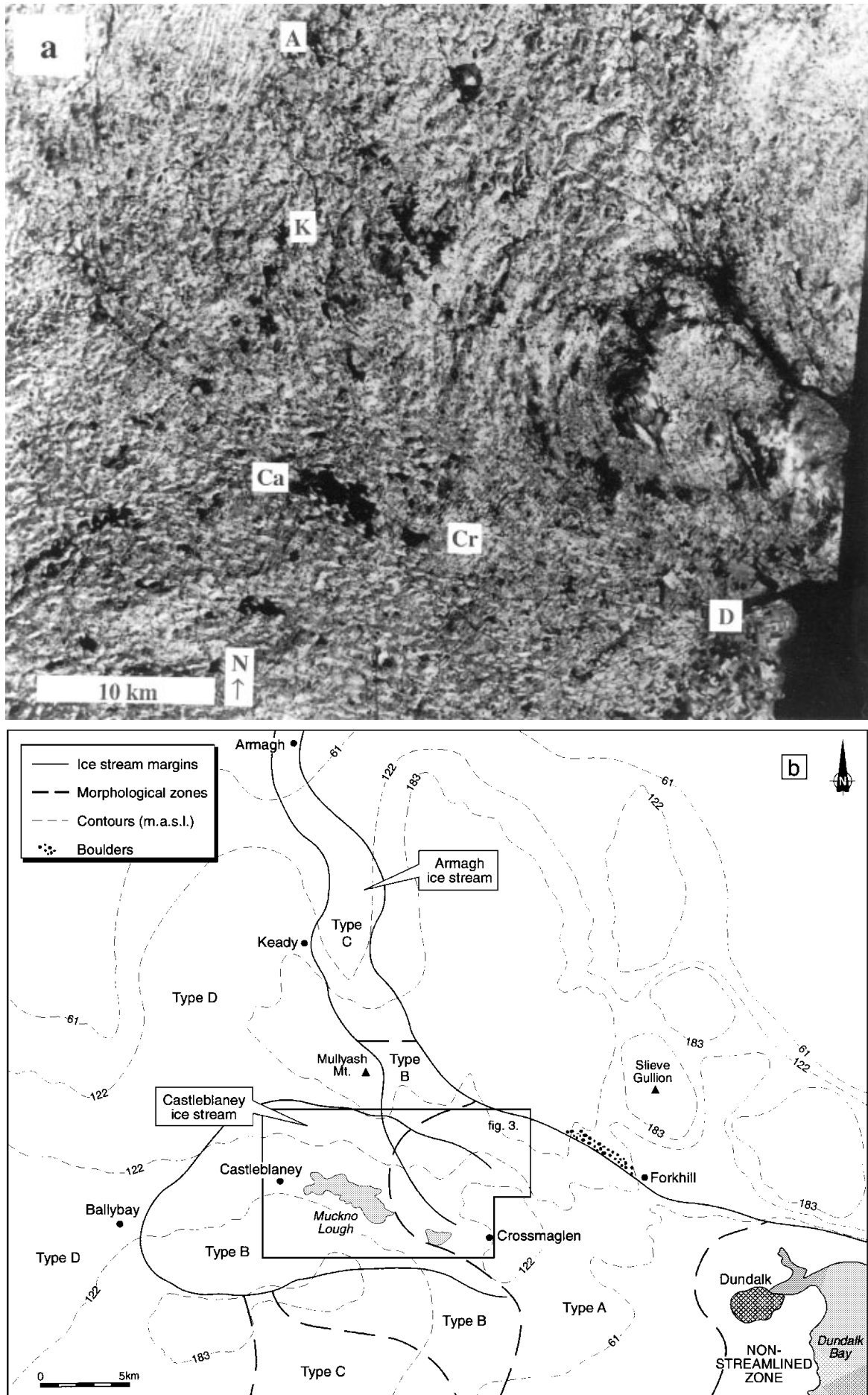
Fig. 2. (a) Landsat TM image (2 May 1990, scene 206/22) showing range of glacial bedform types: D = Dundalk, Cr = Crossmaglen, Ca = Castleblaney, K = Keady, A = Armagh. Striped area west of Armagh is cloud cover. (b) Sketch of same area showing principle topographical features, ice-stream margins and morphological zones A–D.
