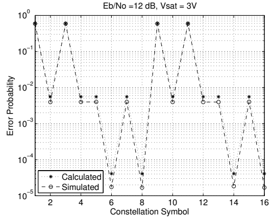
Fig. 6: Individual Symbol Error Probability for 16-QAM with AWGN Channel and Nonlinear PA, V_{SAT} = 3V
