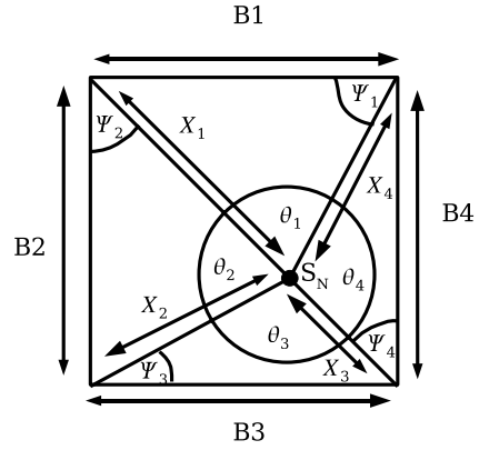
Fig. 3: Signal Point and its Decision Boundaries for M-QAM with a Nonlinear PA and AWGN Channel
