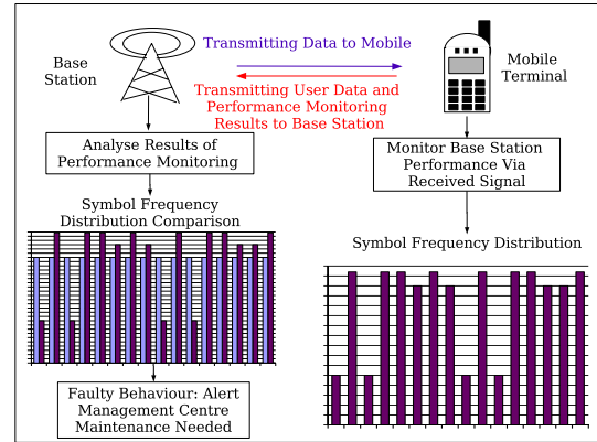
Fig. 1: Proactive Maintenance System Diagram
