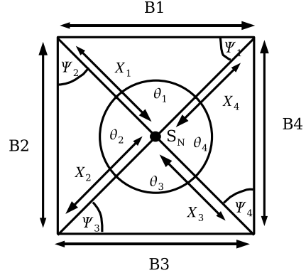
Fig. 2: Signal Point and its Decision Boundaries for M-QAM with AWGN Channel
