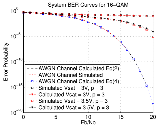
Fig. 4: BER curve for 16-QAM with AWGN Channel and 16-QAM with AWGN Channel and Nonlinear PA
