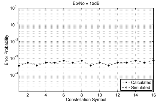
Fig. 5: Individual Symbol Error Probability for 16-QAM with AWGN Channel
