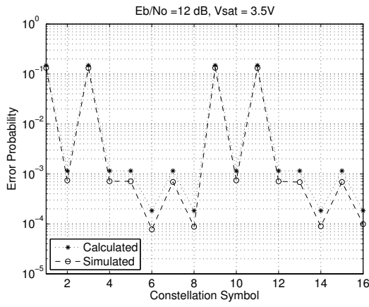
Fig. 7: Individual Symbol Error Probability for 16-QAM with AWGN Channel and Nonlinear PA, V_{SAT} = 3.5V
