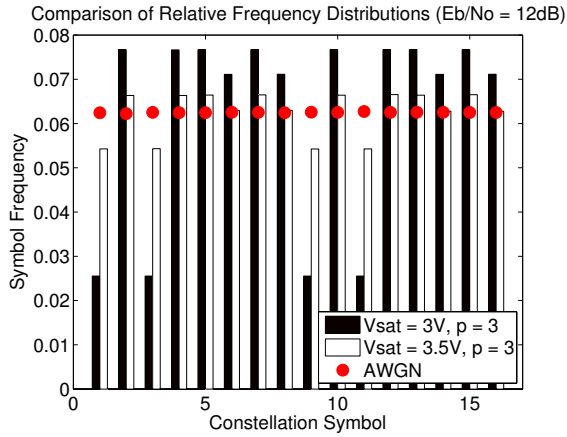
Fig. 8: Comparison of Symbol Frequency for Each Constellation Point for 16-QAM with AWGN Channel and 16-QAM with Nonlinear PA and AWGN channel
