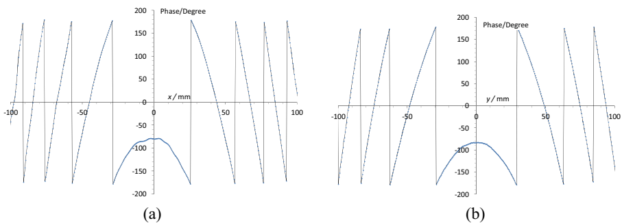
Fig. 5 Reconstructed phase front for HUT at scan plane using digital holography. a x-cut and b y-cut near center of the field
