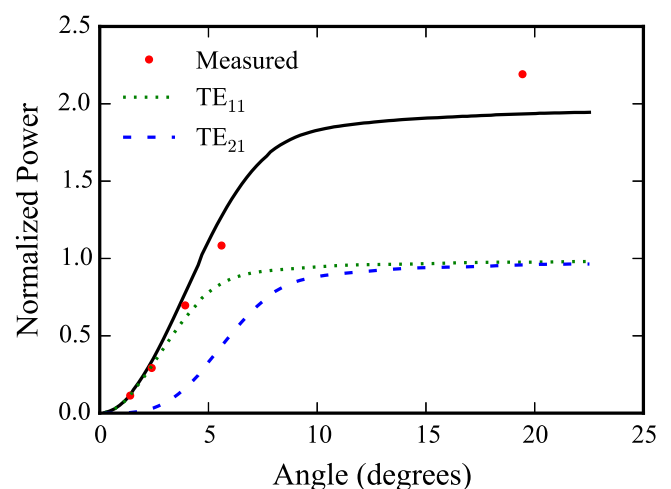
FIG. 11. Measured optical power at T_{BB} = 26 K vs source angular size, compared with the expected encircled power derived from the far-field beam patterns of the TE_{11} and TE_{21} modes shown in Figure 9. The solid line shows the sum of the encircled powers expected for the TE_{11} and TE_{21} modes. There is good agreement for small angular size and the model underestimates the power for the large aperture due to the off-axis contribution of higher-order modes.
