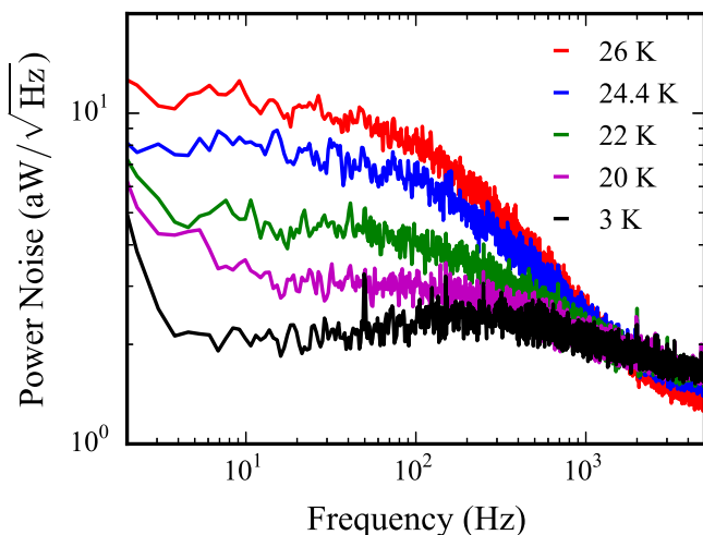
FIG. 5. Example of detector power noise measured with different black-body illuminator temperatures. This power noise is derived by multiplying the current noise by the TES voltage, and is equal to the NEP for low frequencies (compared with the detector bandwidth). The lowest curve with the illuminator at its base temperature (3 K) shows the intrinsic noise of the detector with negligible incident optical power. For high illuminator temperatures the photon shot noise dominates and the speed of the detector is reduced.
