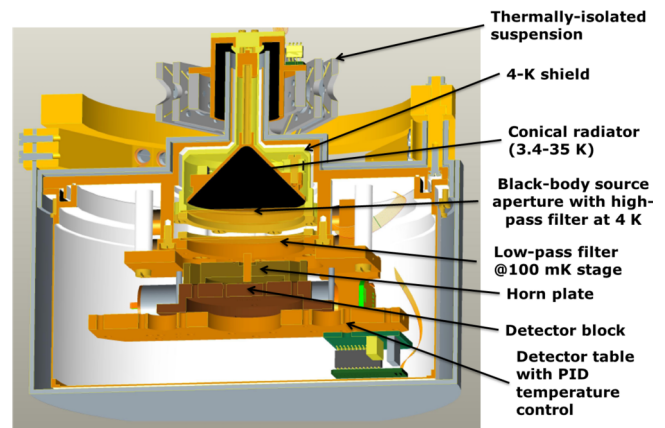
FIG. 4. Cross-section of a light-tight, magnetically shielded experiment box. The conical black-body radiator illuminates the detector through a 12-mm diameter aperture in the shield. The box is heatsunk to the mixing chamber of the dilution refrigerator. Reproduced with permission from Audley et al. , J. Low Temp. Phys. 176 , 755 (2014). Copyright 2014 Springer.
