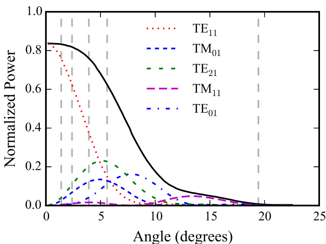
FIG. 9. Far-field power patterns of the circular waveguide modes supported by the feedhorn in the passband of the filter stack. The vertical dashed lines show the angles subtended by the different apertures placed in front of the black-body source. From left to right, these are 0.5, 0.9, 1.4, and 2.0, and 12 mm; the rightmost vertical dashed line corresponds to the case where the 12-mm diameter illuminator is unobscured and it essentially fills the beam of the horn. Note that only the fundamental TE_{11} mode has significant on-axis power.
