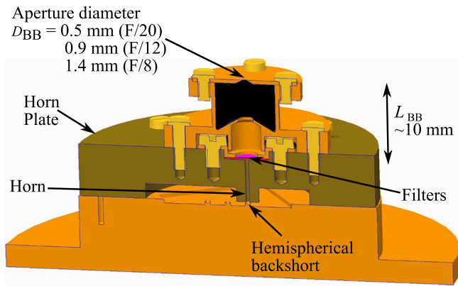
FIG. 8. Cross-section of detector holder with can for varying pinhole diameter mounted in front of the feedhorn. The top plate contains a beam-defining pinhole and can be exchanged to change the pinhole diameter, D_{BB} . This allows us to make measurements with beams of different angular size to investigate the effects of higher-order modes.
