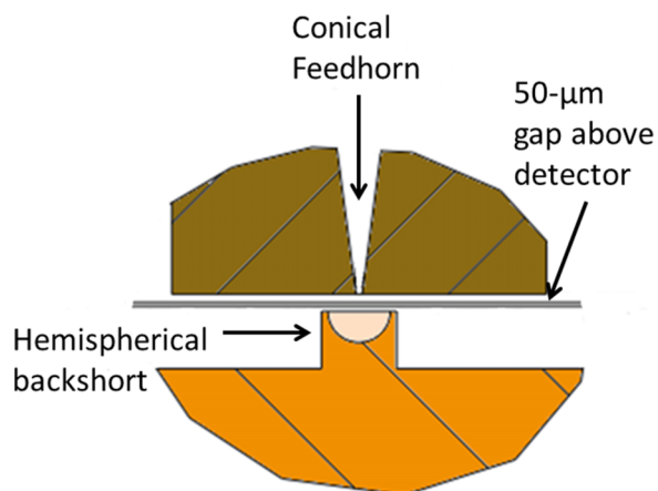
FIG. 2. A cross-section showing the optical coupling scheme. 9 The TES bolometer sits between a conical feedhorn and a hemispherical backshort. The exit aperture of the feedhorn is 46 \mu\text{m} in diameter and the diameter of the hemispherical backshort is 500 \mu\text{m} . Both the feedhorn and the backshort are made of copper. Reproduced with permission from Audley et al. , Proc. SPIE 9153 , 91530E (2014). Copyright 2014 Society of Photo Optical Instrumentation Engineers.
