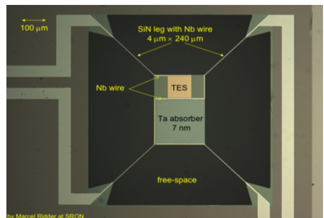
FIG. 1. A TES bolometer of the type measured. The TES and Ta absorber sit on a 1- \mu\text{m} thick SiN membrane. The membrane is supported by four thin legs which provide a weak thermal link to the substrate and carry superconducting Nb tracks for electrical connection. Reproduced with permission from Audley et al. , J. Low Temp. Phys. 176 , 755 (2014). Copyright 2014 Springer.
