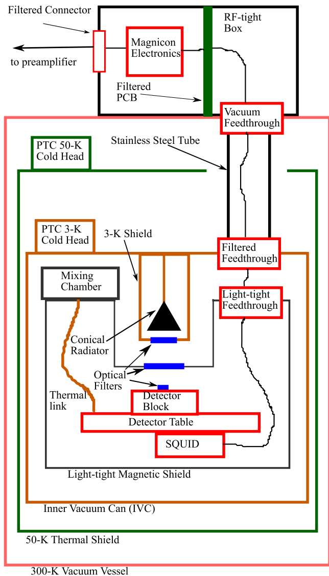
FIG. 3. Simplified schematic diagram of the test facility. The inner vacuum can, which is heatsunk to the 3-K cold head of the pulse-tube cooler (PTC), and the main vacuum vessel form Faraday cages. The detectors and their SQUID readout sit on a temperature-stabilized table inside a light-tight magnetic shield that is heatsunk to the mixing chamber of the dilution refrigerator.
