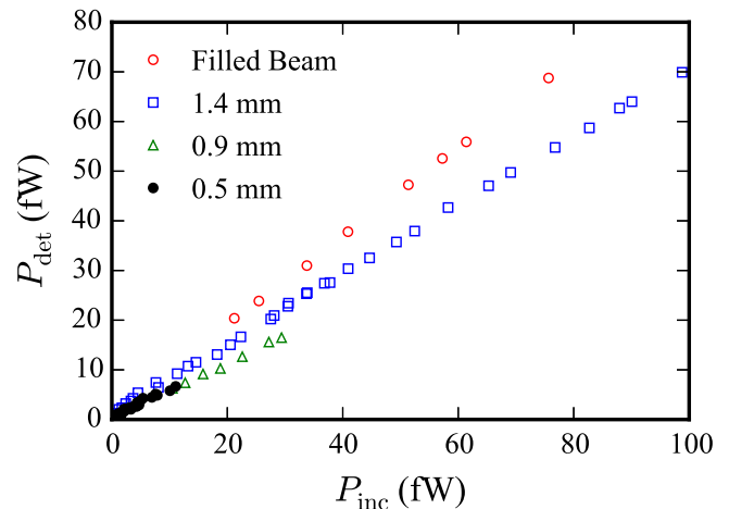
FIG. 10. Optical power detected by the bolometer, P_{det} , vs the incident optical power, P_{inc} . Pinholes of diameter 0.5, 0.9, and 1.4 mm were placed in front of the feedhorn to reduce the angular size of the source. The case where the source fills the beam of the feedhorn (no pinhole) is also shown. If we assume that a single mode propagates in the feedhorn, the apparent optical efficiency is 88% for the filled beam and 60% for the two smallest pinholes.
