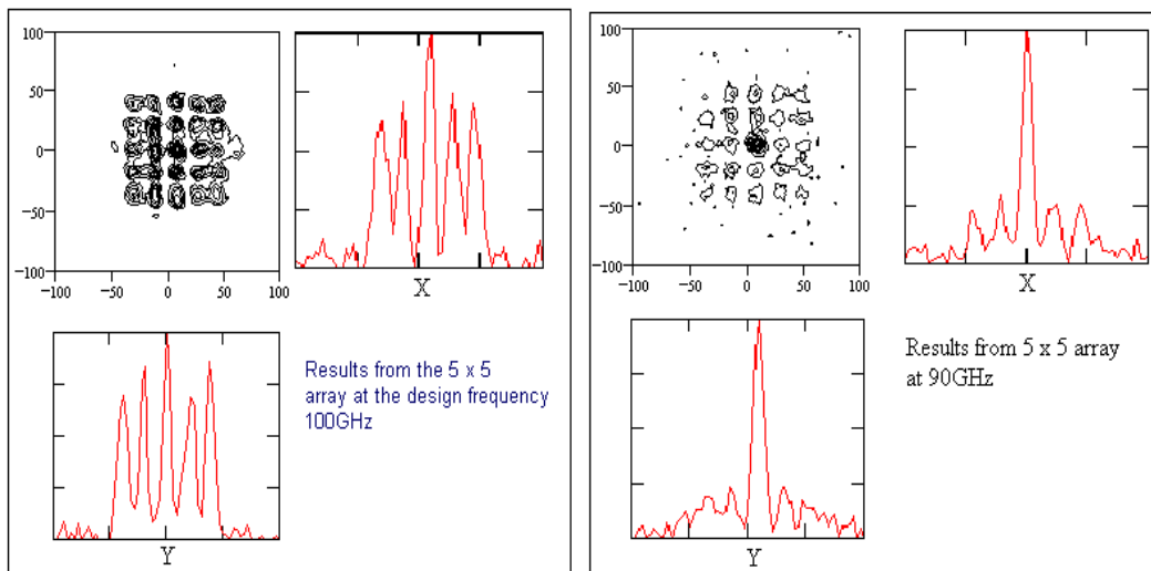
Results for the 5 \times 5 array at the centre frequency and beyond the band limit.
